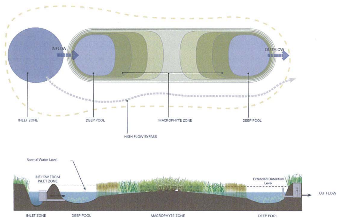
Figure 9 Typical constructed wetland details (source: Water by Design)
