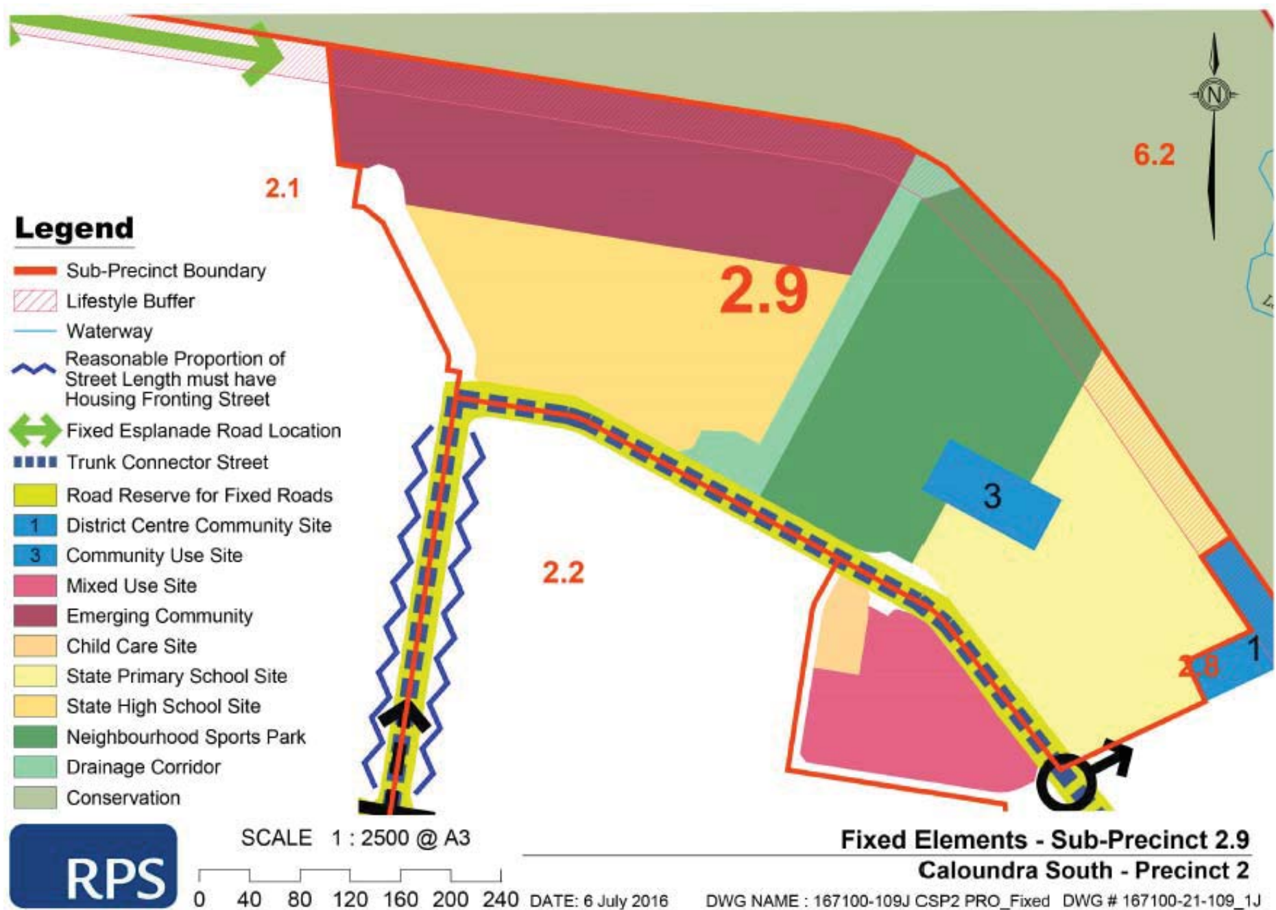
FIGURE 10 – SUB PRECINCT 2.9 FIXED ELEMENTS
