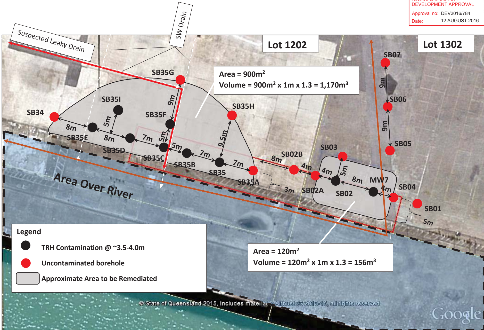
Figure 1 – Site Plan Showing Borehole Locations and Extent of TRH Remediation 0 10m SCALE
