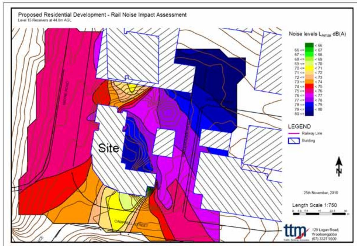
Figure 11: Noise Contour Map L_{A\text{Max}} – Level 15.
