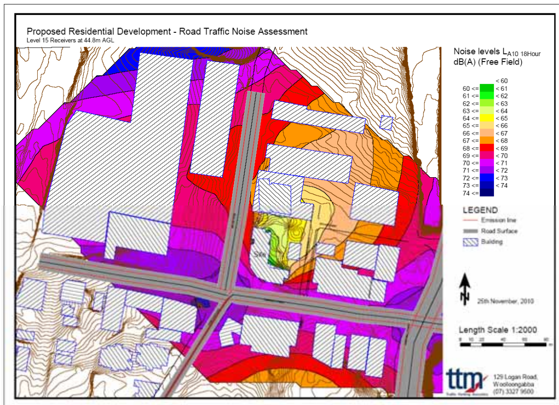
Figure 7: Noise Contour Map L_{A10,18\text{hour}} – Level 15.
