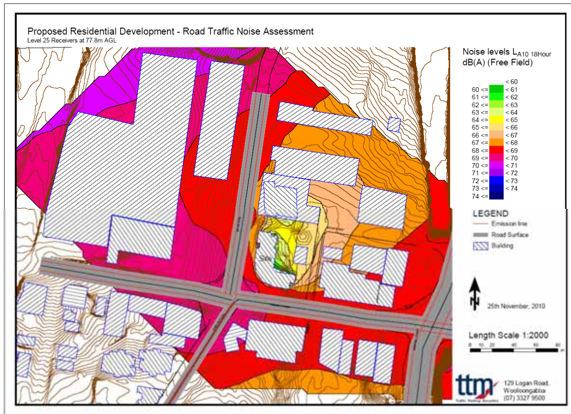
Figure 8: Noise Contour Map L_{A10,18\text{hour}} – Level 25.
