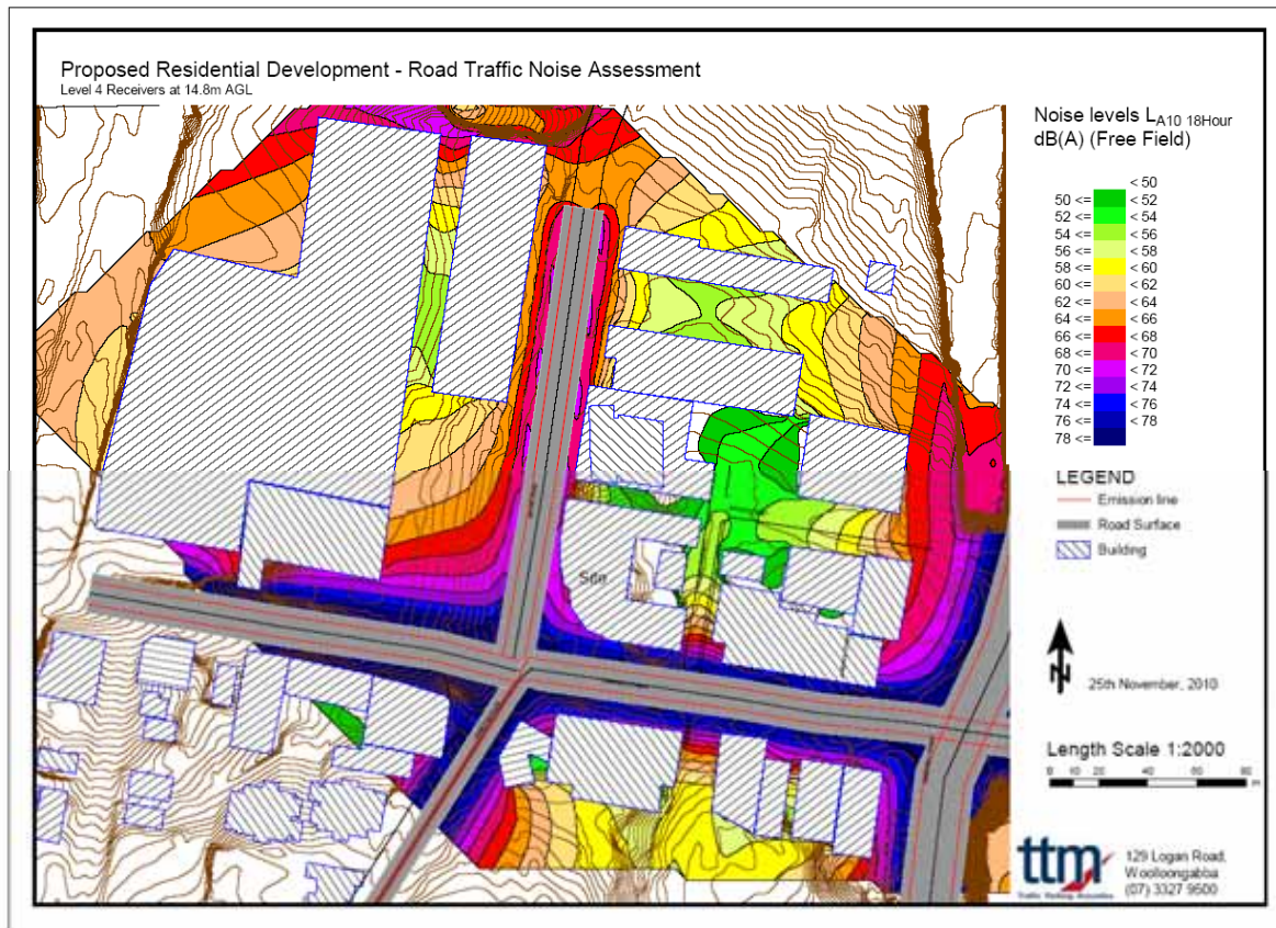
Figure 6: Noise Contour Map L_{A10,18\text{hour}} – Level 4.
