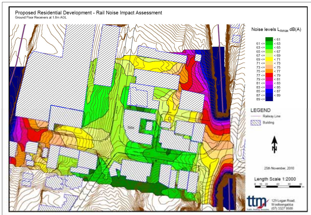
Figure 9: Noise Contour Map L_{Amax} – Ground Level.
