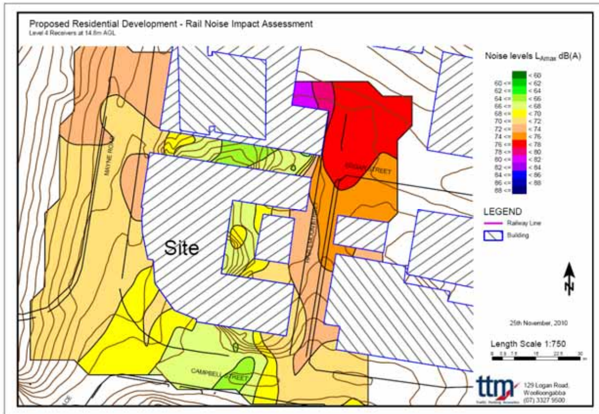
Figure 10: Noise Contour Map L_{A\text{Max}} – Level 4.
