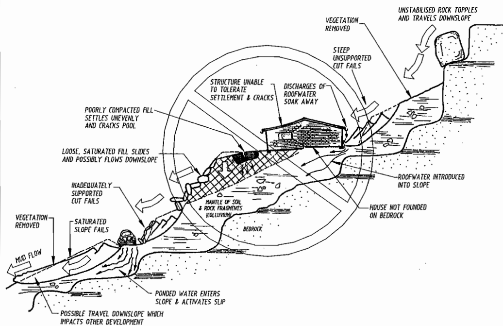
FIGURE J1: Illustrations of Good and Poor Hillside Practice
