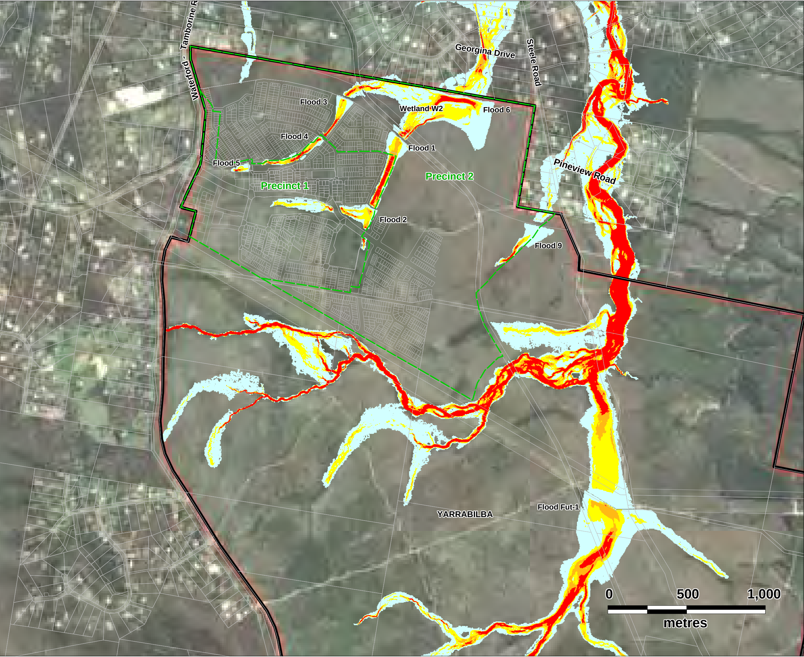
FIGURE D4 Post-Development (Mitigated) 100 year ARI Velocity x Depth
