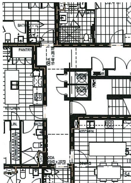
Figure 8.1.1 Accommodation level twin garbage shoots
