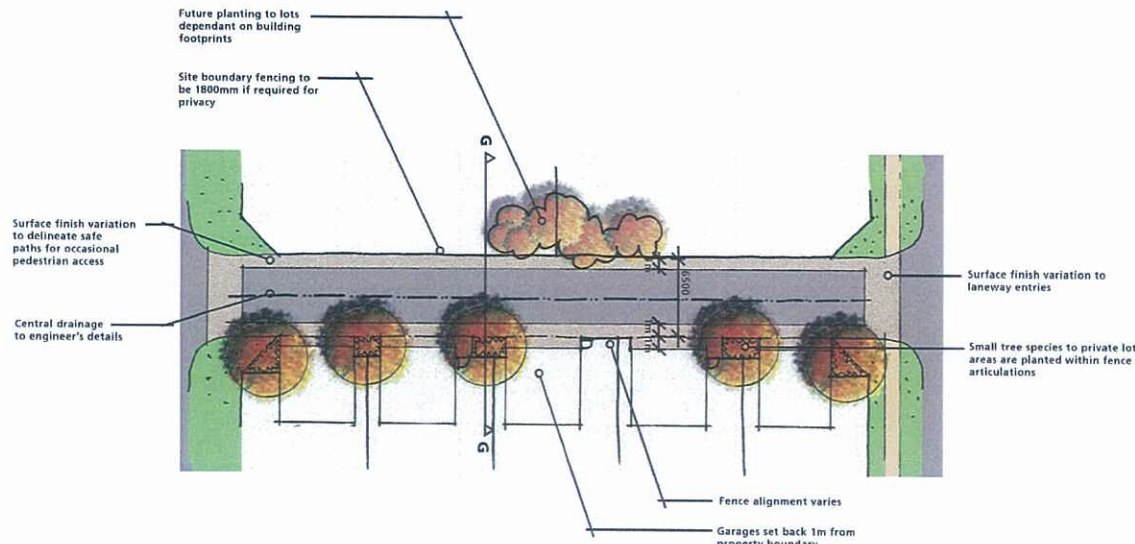
DETAIL D - TYPICAL LANEWAY TREATMENTS 1:200 AT A1
