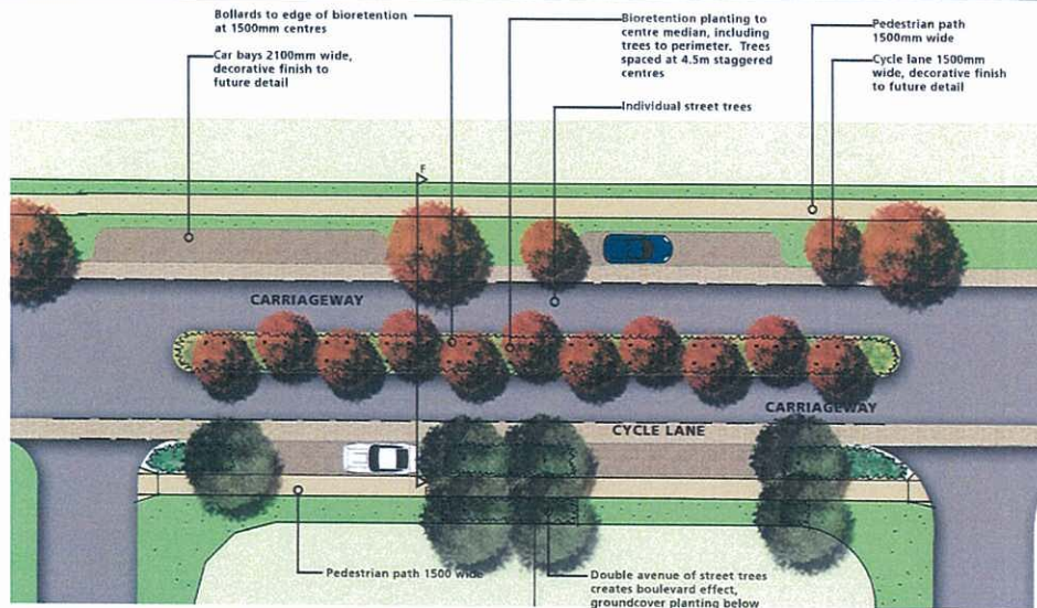
DETAIL C - TYPICAL ROAD 1 TREATMENTS 1:200 AT A1
