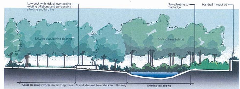
SECTION H-H 1:100 AT A1
