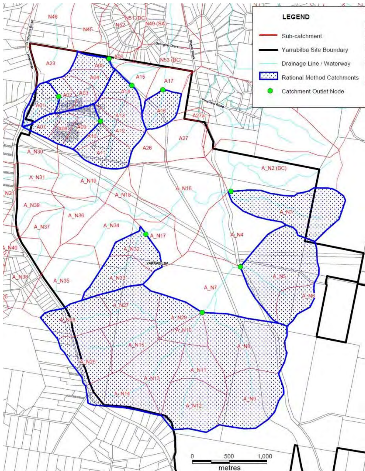
Figure A1: Pre-development Rational Method catchments and discharge locations
