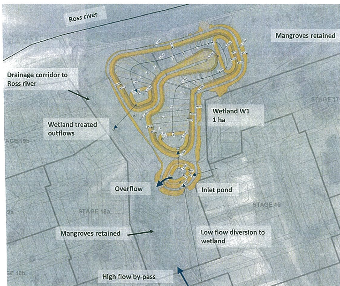
Figure 13 Preliminary earthworks model - wetland W1
