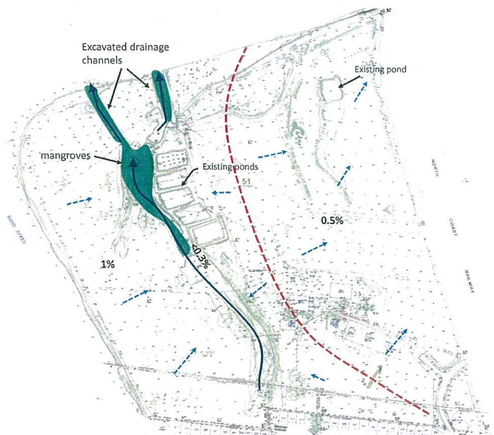
Figure 3 General drainage, catchments and topography
