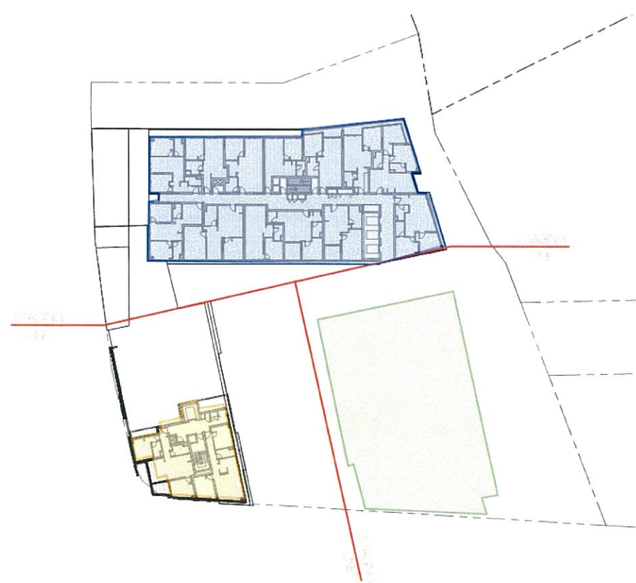
LEVEL 7 AND ABOVE NTS
