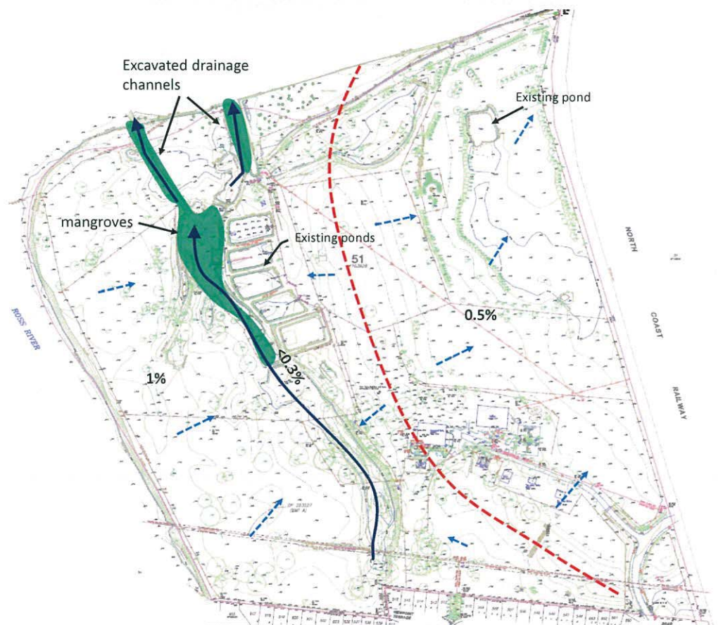
Figure 3 General drainage, catchments and topography
