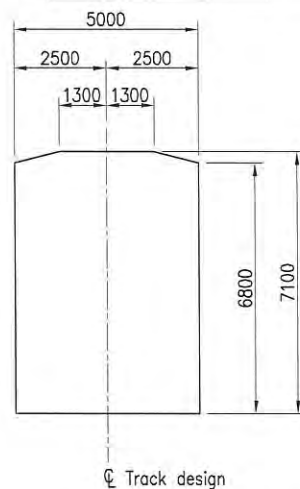
CLEARANCE ENVELOPE TYPE 1 Scale A
