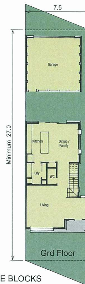
TERRACE BLOCKS
