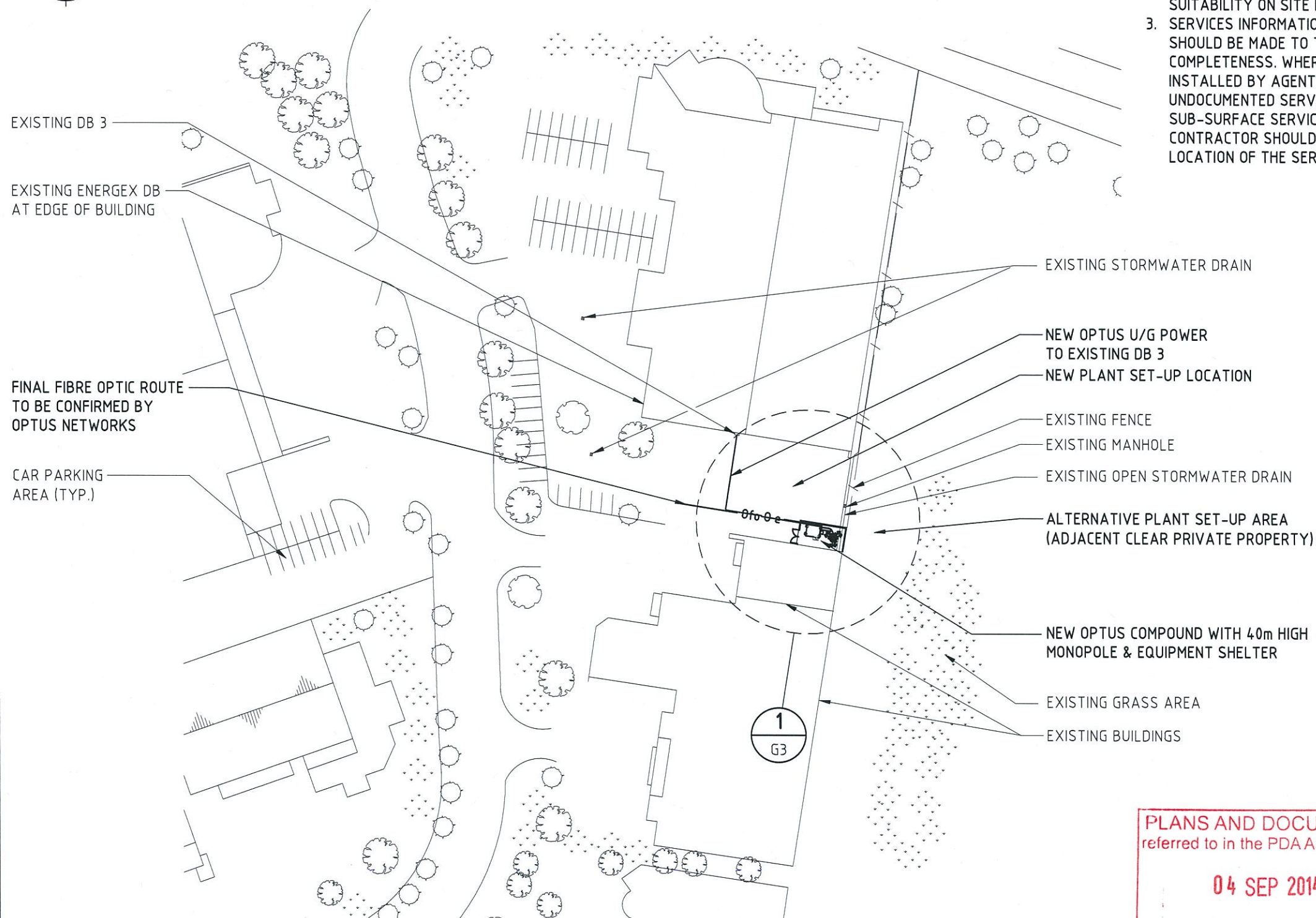
OVERALL SITE PLAN SCALE 1:1000
