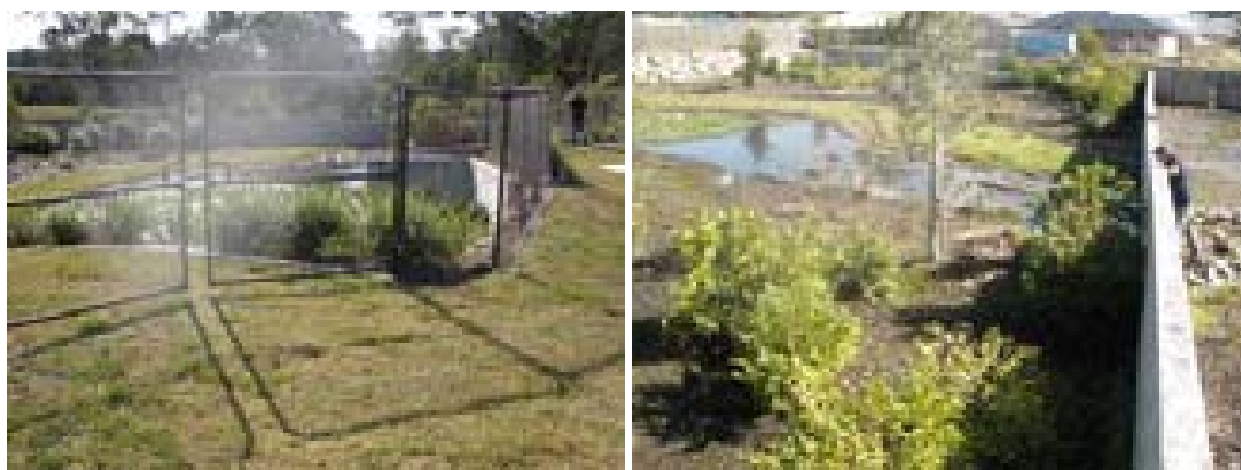
Figure 4-2 Example of a Poorly Integrated 'End-of-Pipe' Bioretention Basin
