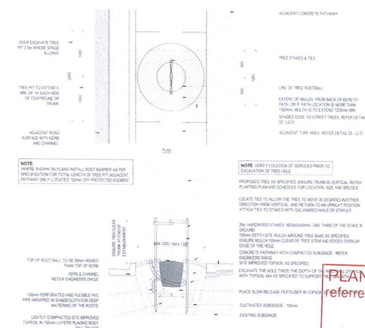
Typical Street Tree Planting Detail - NTS
