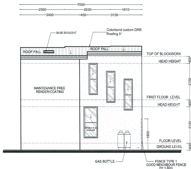
ELEVATION 3 SCALE 1:100
