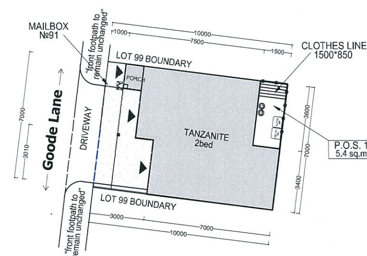
○ FENCE PLAN SCALE 1:200
