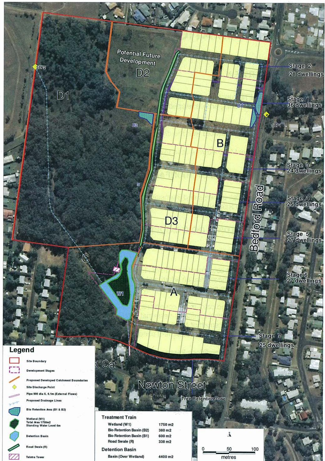
Figure 2.3 Proposed Developed Conditions and Stormwater Management Measures
