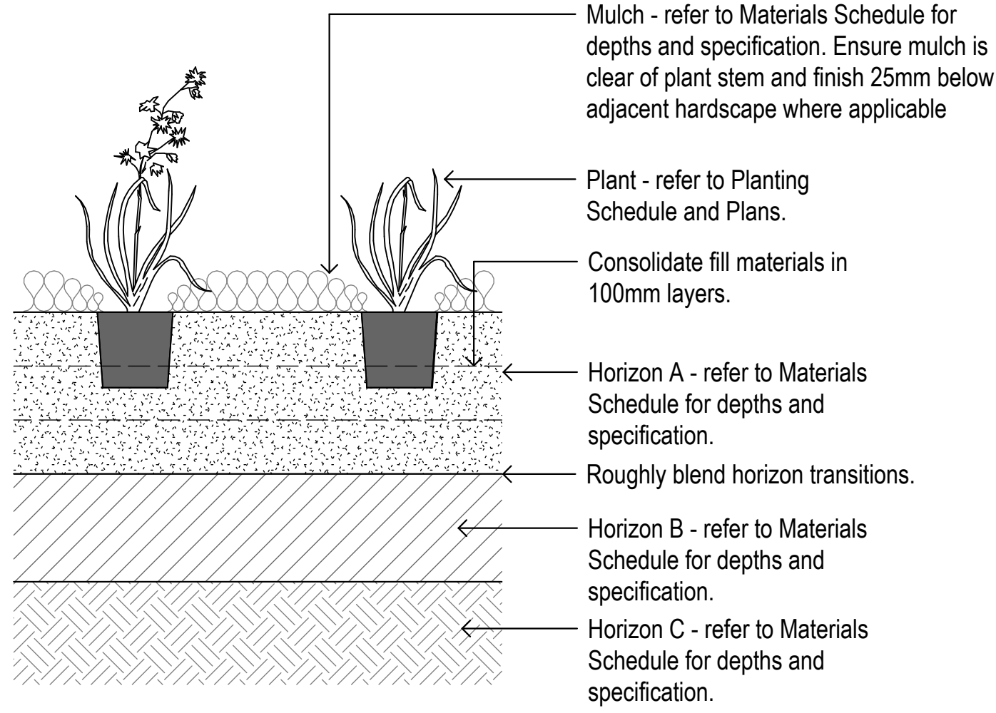
PA1 GF - TYPICAL PLANTING - PA1 SCALE - 1 : 10 @ A1
