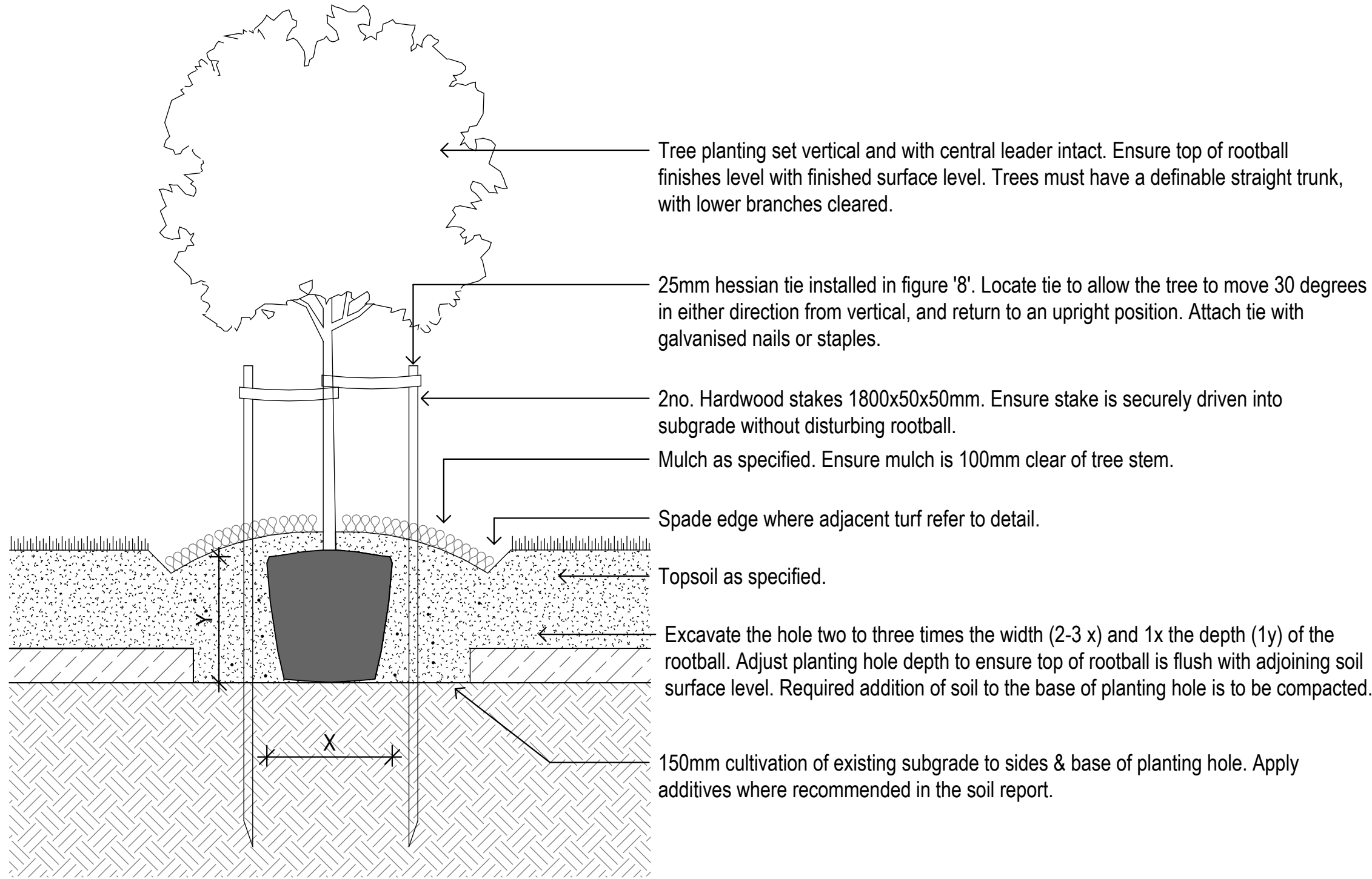
2 TYPICAL TREE PLANTING IN TURF AREA SCALE - 1 : 20 @ A1
