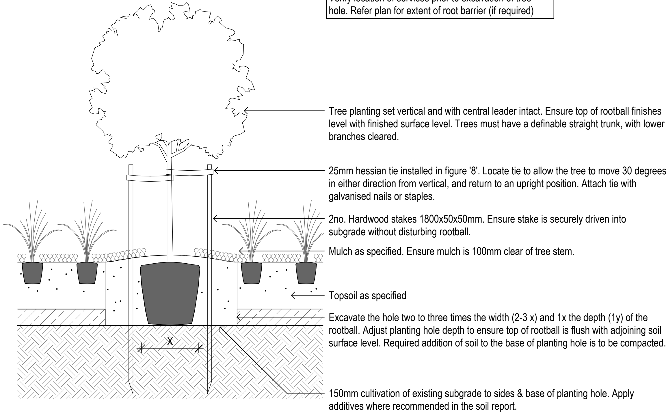
1 TYPICAL TREE PLANTING IN PLANTING AREA SCALE - 1 : 20 @ A1
