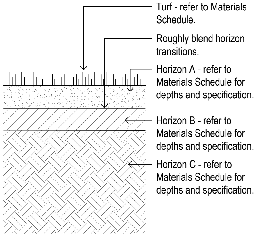
TF1 GF - TYPICAL TURF - TF1 SCALE - 1 : 10 @ A1
