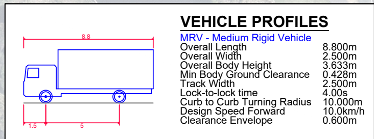
8.80m MRV ACCESS AND EGRESS FROM THE SITE SCALE 1:1000
