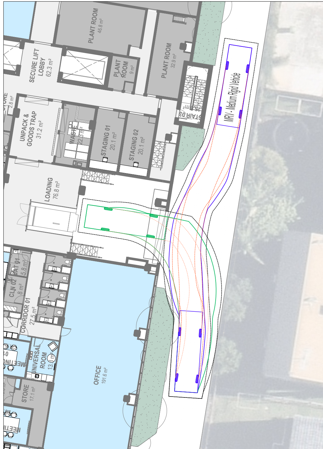
8.80m MRV ACCESS THE LOADING ZONE SCALE 1:250
