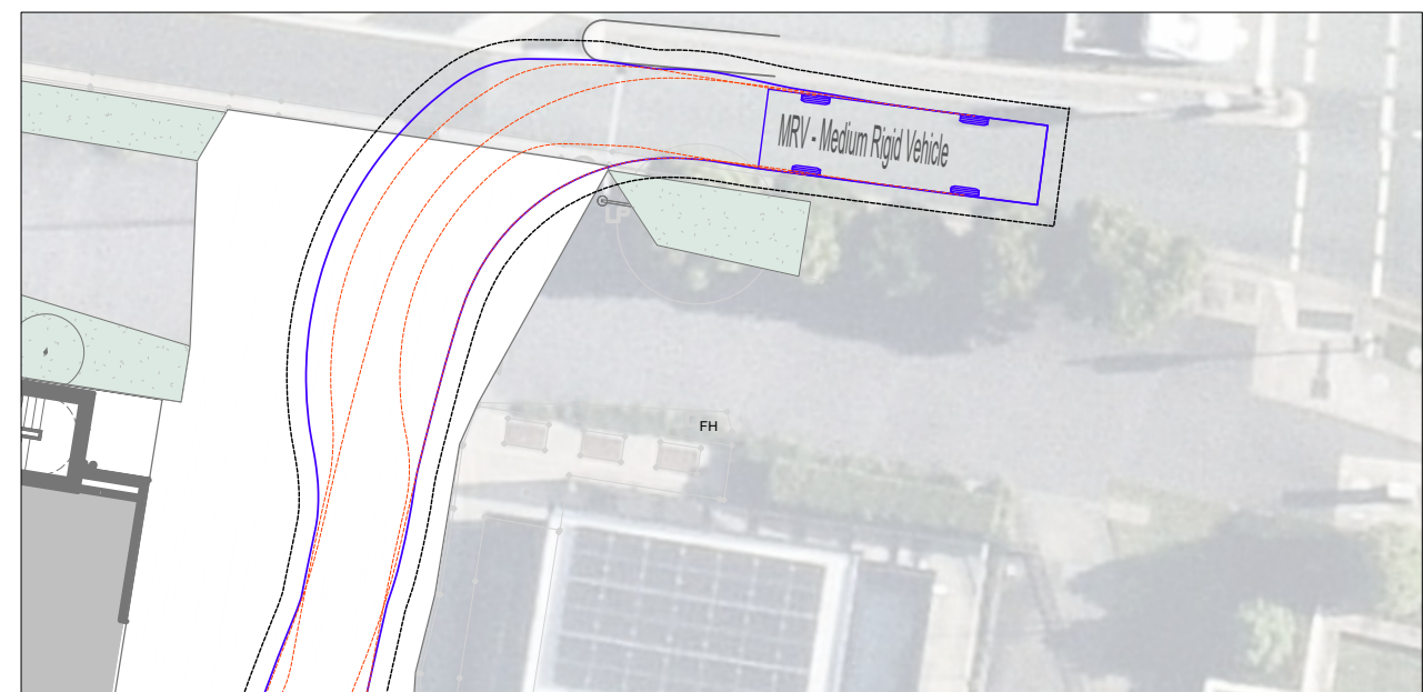
NORTH ACCESS DRIVEWAY LAYOUT SCALE 1:250
