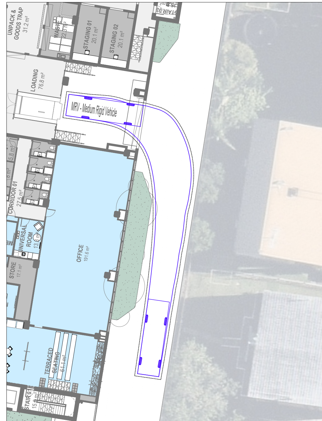
8.80m MRV EGRESS FROM THE LOADING ZONE SCALE 1:250
