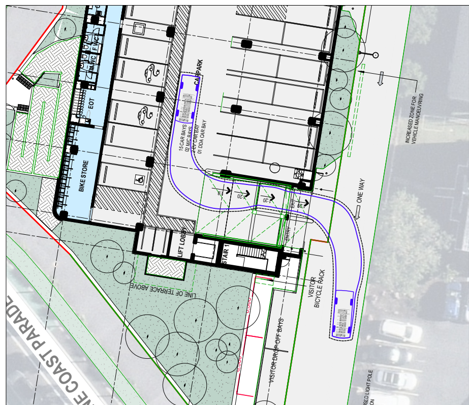
B99 CAR ACCESSING AND EGRESSING FROM THE SITE
