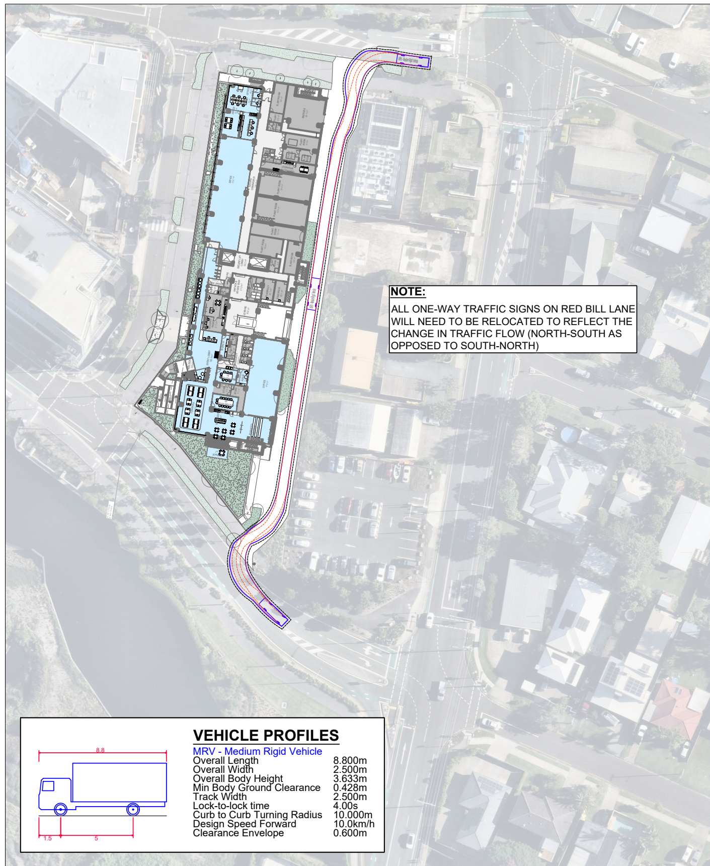
8.80m MRV ACCESS AND EGRESS FROM THE SITE SCALE 1:1000
