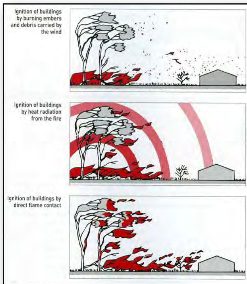
Figure 10. Main Bushfire Attack mechanisms (Image courtesy of Ramsay & Rudolf, 2003)
