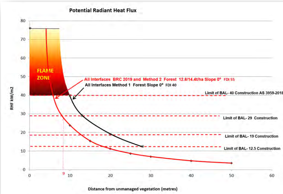
Figure 11. Radiant Heat Flux Predicted by Methods 1 and 2.
