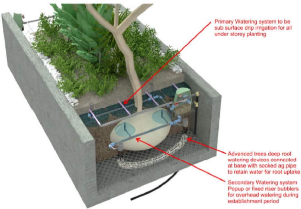
The "hybrid" irrigation system for contained planters and podium planted areas is highly recommended to provide the flexibility of additional overhead watering for fast plant establishment
