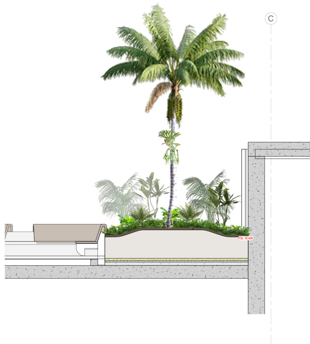
1 Level 2 - Section 1 LS-200-L02-00 1 : 25
