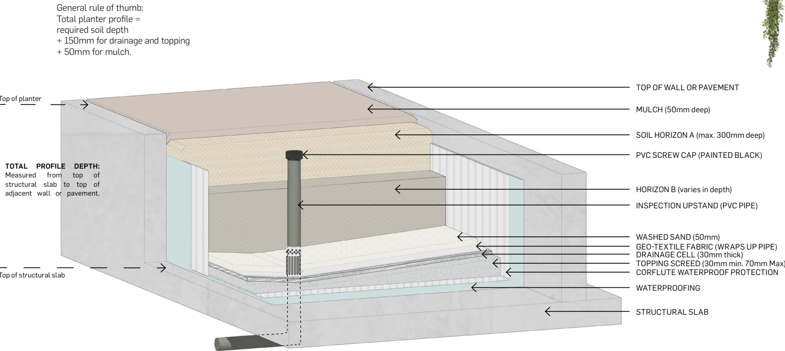
TYPICAL ON-STRUCTURE PLANTER BUILD-UP
