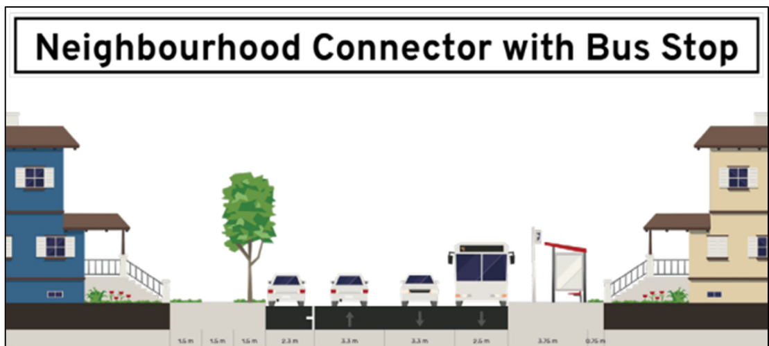
Figure 2.4: NEIGHBOURHOOD CONNECTOR CROSS SECTION
