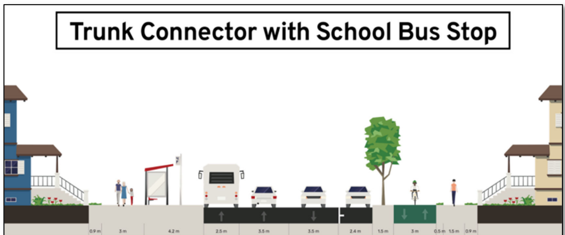
Figure 2.5: TRUNK CONNECTOR CROSS SECTION WITH SCHOOL BUS STOP
