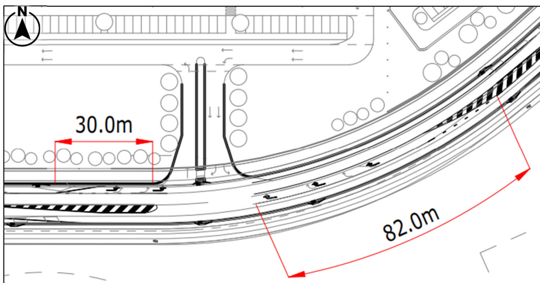
Figure 4.2: CONCEPT SITE ACCESS LAYOUT
