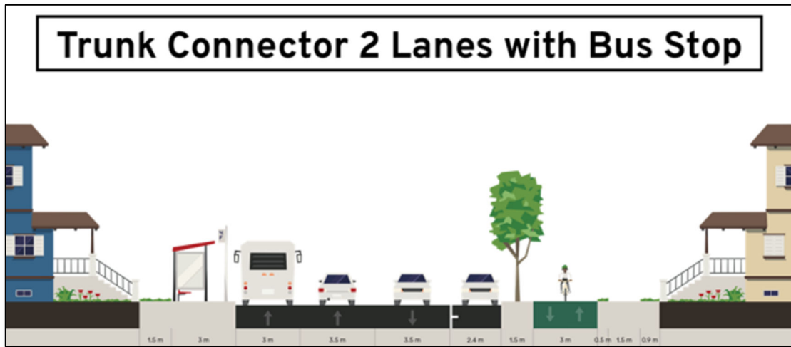
Figure 2.3: TRUNK CONNECTOR CROSS SECTION
