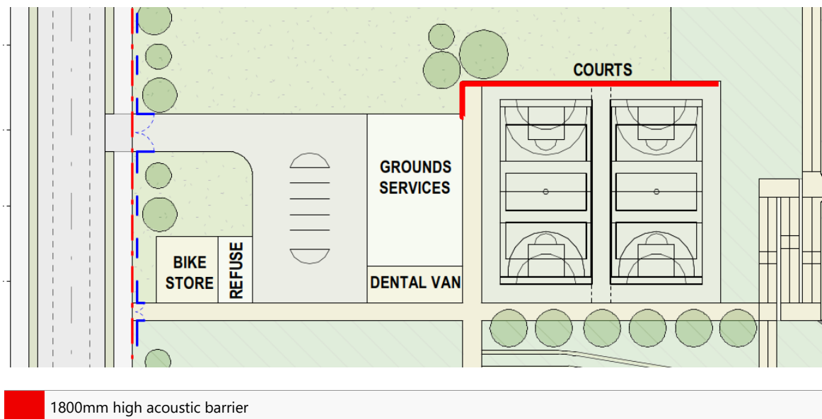
Figure 6-2: Acoustic screen around courts RENZO TONIN & ASSOCIATES New Primary School in Greater Flagstone Noise Impact Assessment
