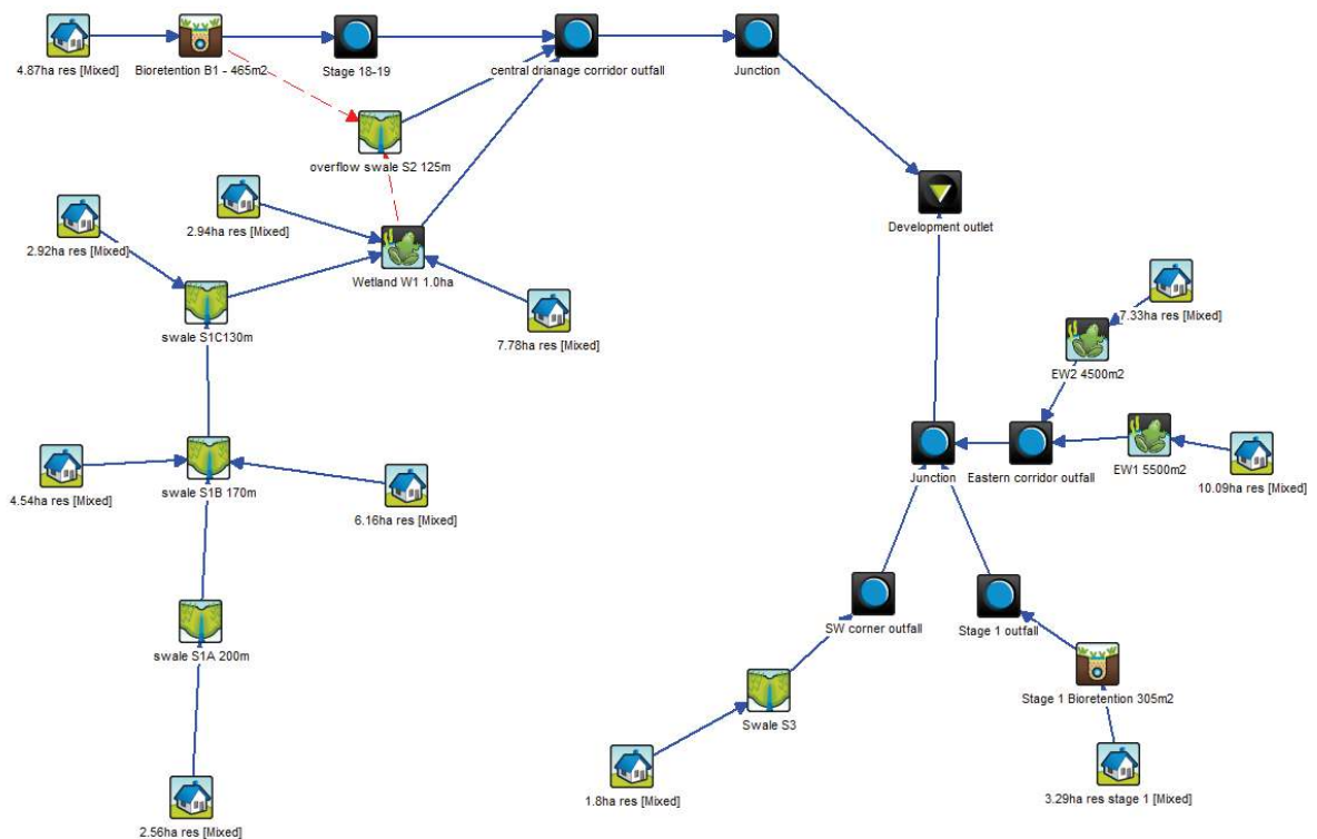
Figure 12: MUSIC catchment and model layout
