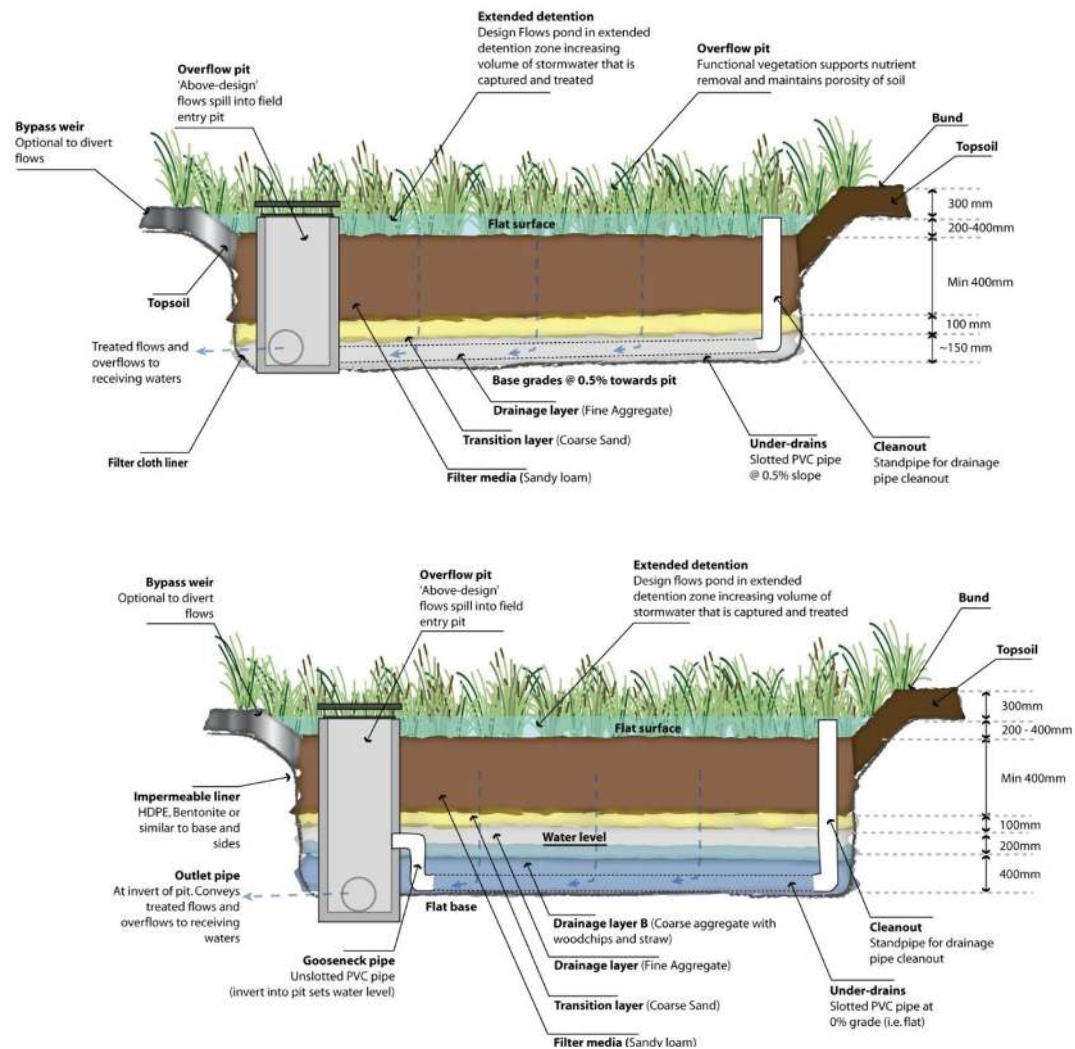
Figure 11: Typical section through bio-retention basin with a saturated zone
