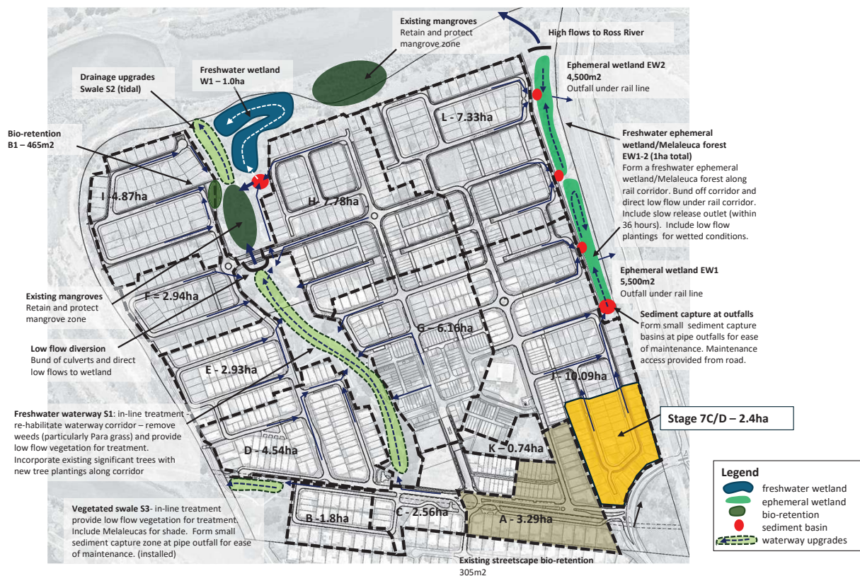
Figure 2 – Approved stormwater quality management strategy with Stages 7c and D shown
