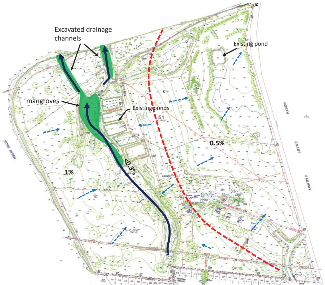
Figure 3 General drainage, catchments and topography
