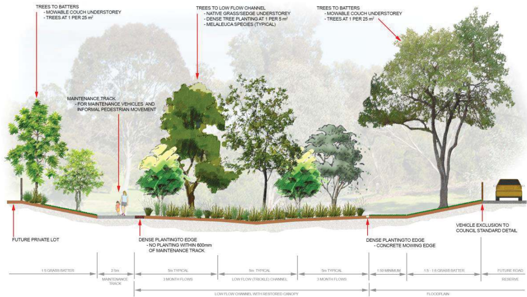
Figure 7 Typical section of a naturalised waterway
