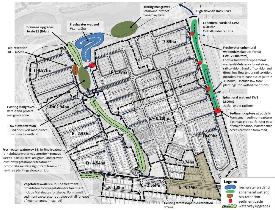
Figure 6 Oonoomba stormwater treatment strategy
