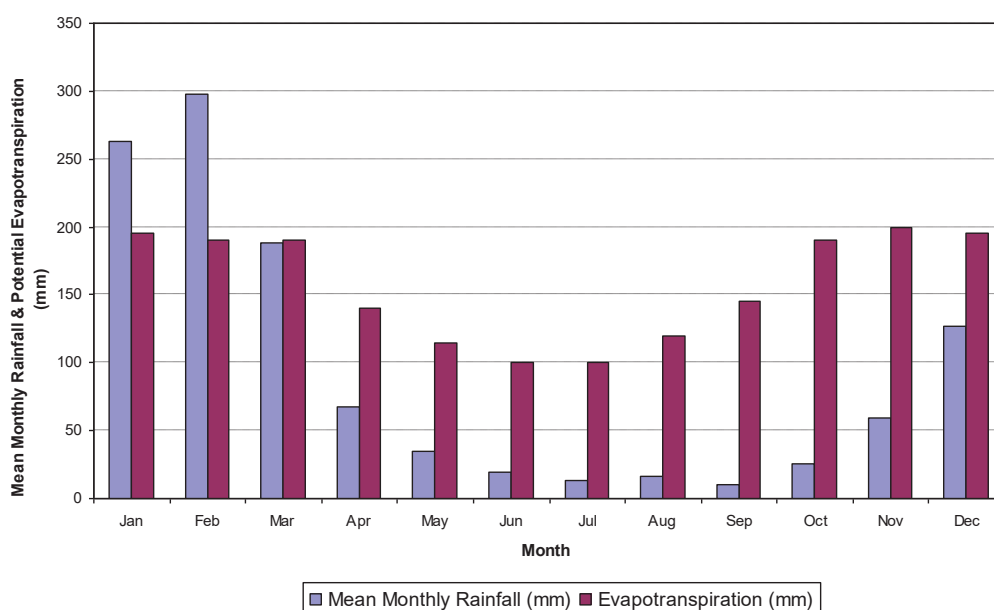
Figure 2: Average climate data for Townsville
