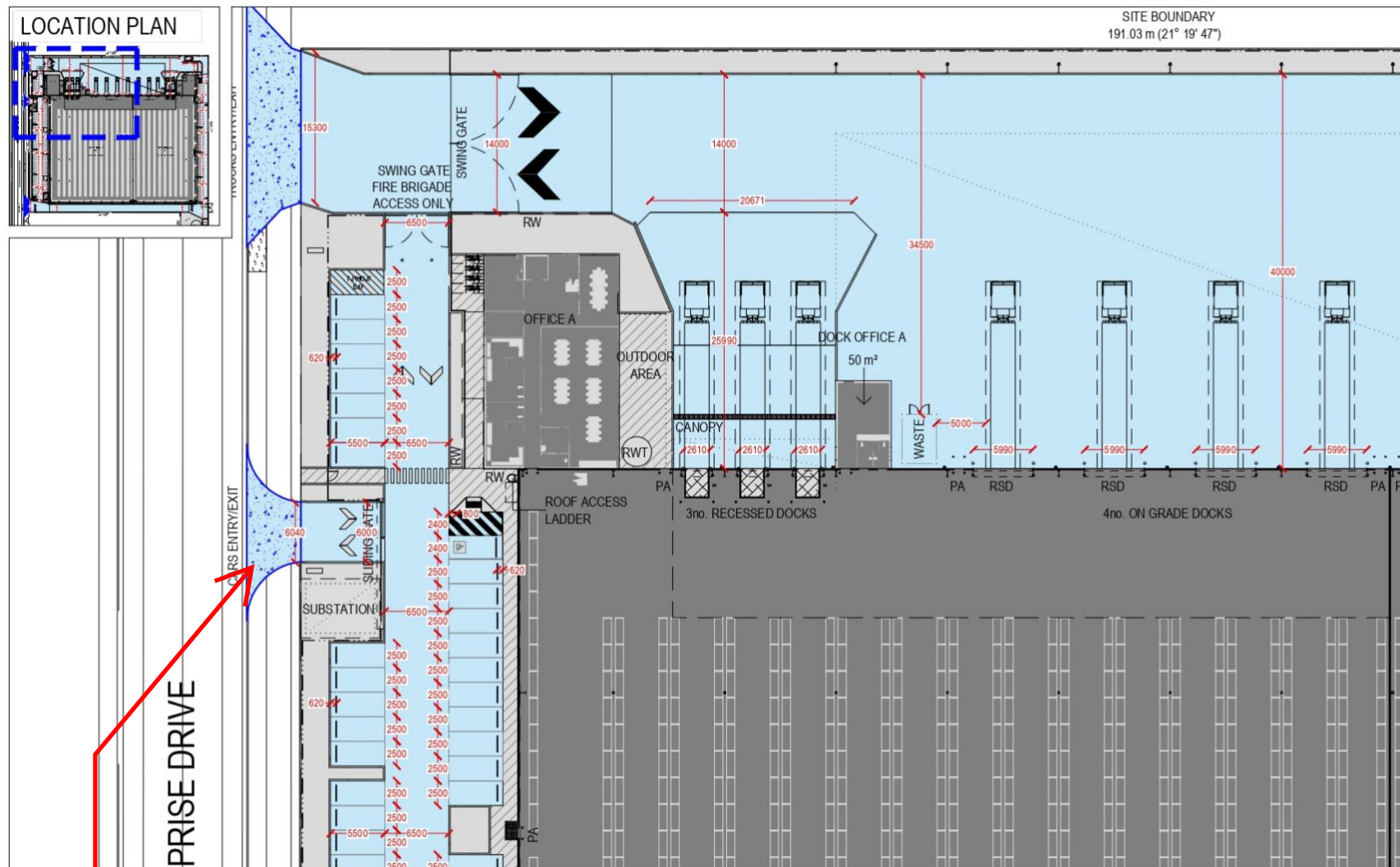
FIGURE 4.4 – PROPOSED CAR PARKING LAYOUT AND DIMENSIONS
