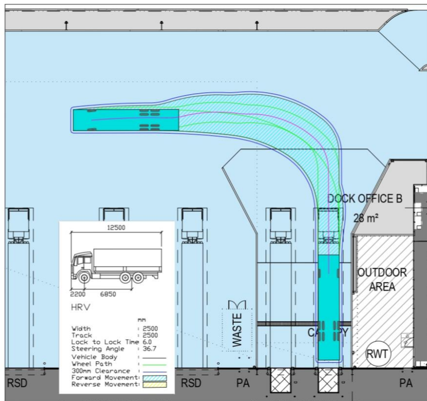
FIGURE 6.2 –SWEEP PATHS FOR HEAVY RIGID VEHICLE (HRV)
