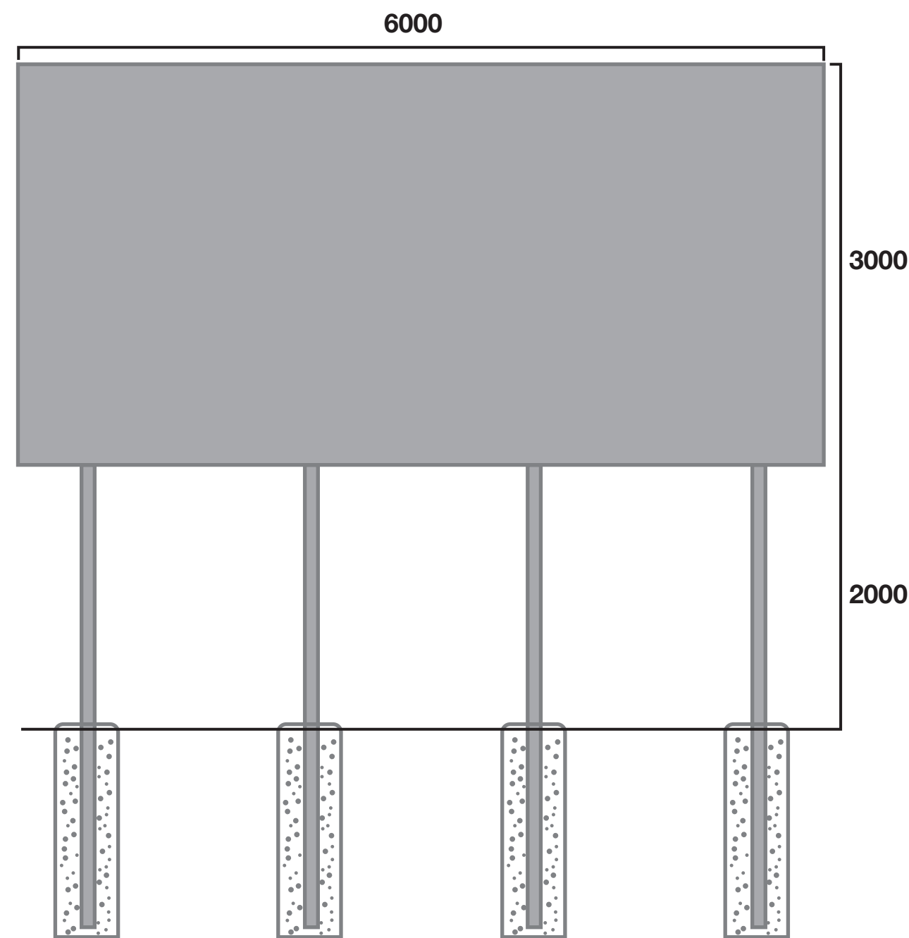
Front View
