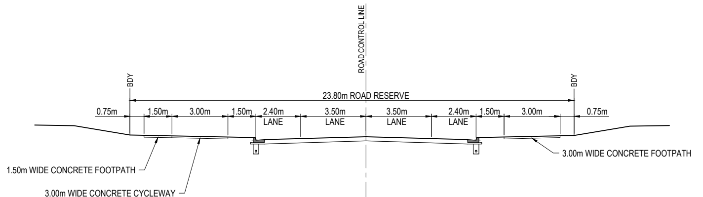
23.80m ROAD RESERVE - TYPICAL SECTION
