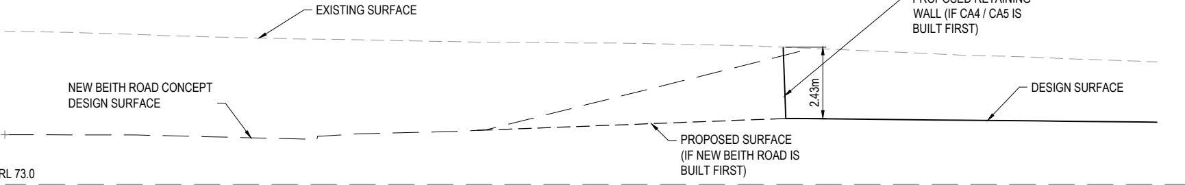
SECTION 3 SCALE 1:100 (A1) SCALE 1:200 (A3)
