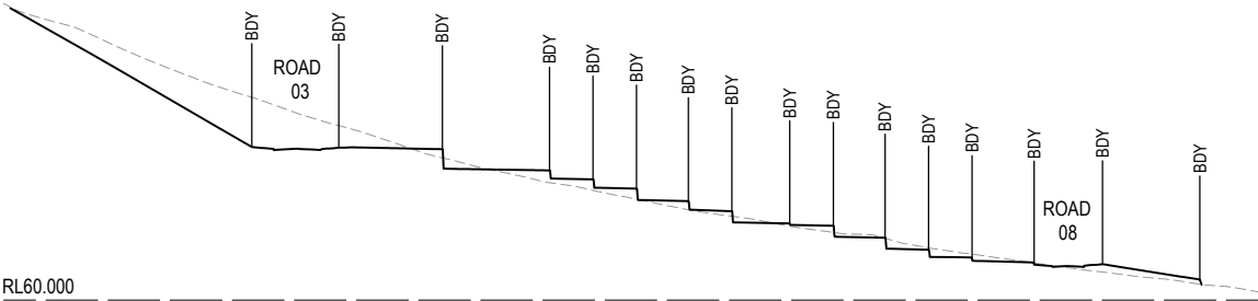
RL60.000 SECTION L SCALE 1:1000 (H) SCALE 1:500 (V)
