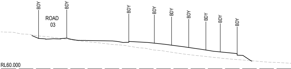
RL60.000 SECTION K SCALE 1:1000 (H) SCALE 1:500 (V)
