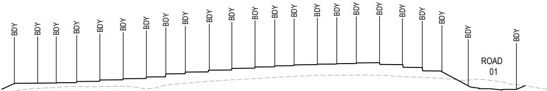
RL60.000 SECTION J SCALE 1:1000 (H) SCALE 1:500 (V)
