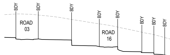
SECTION E SCALE 1:1000 (H) SCALE 1:500 (V)
