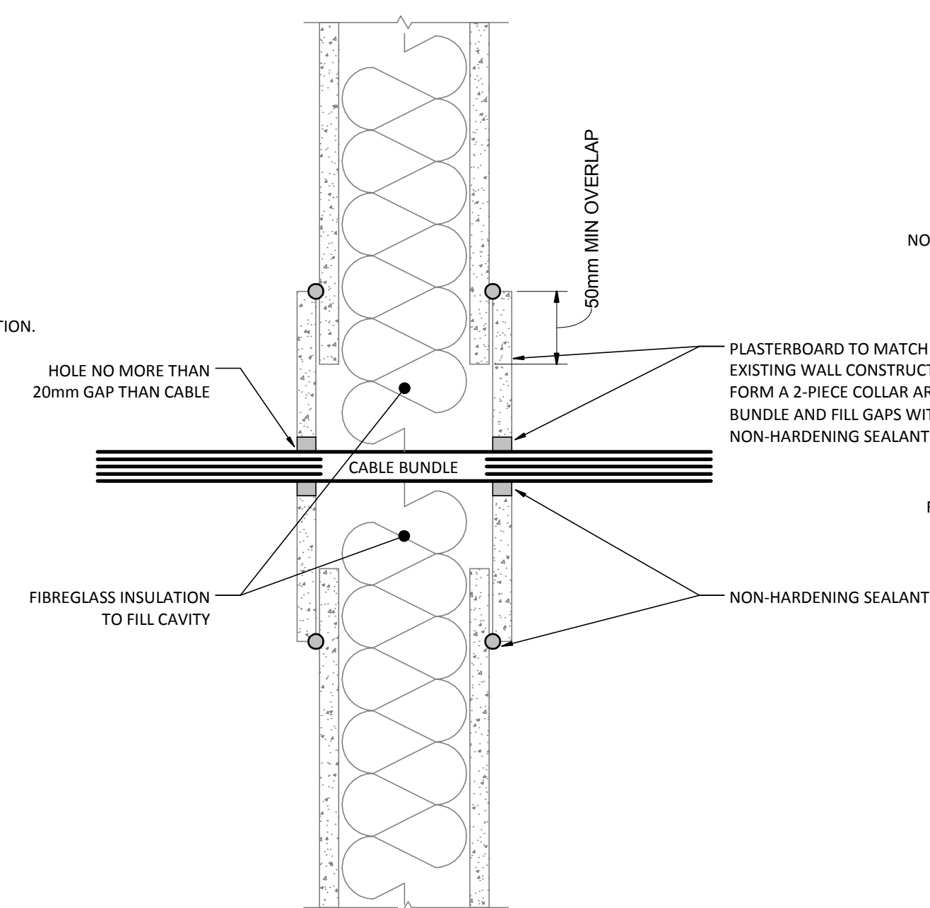
4 CABLE PENETRATION NOT TO SCALE
