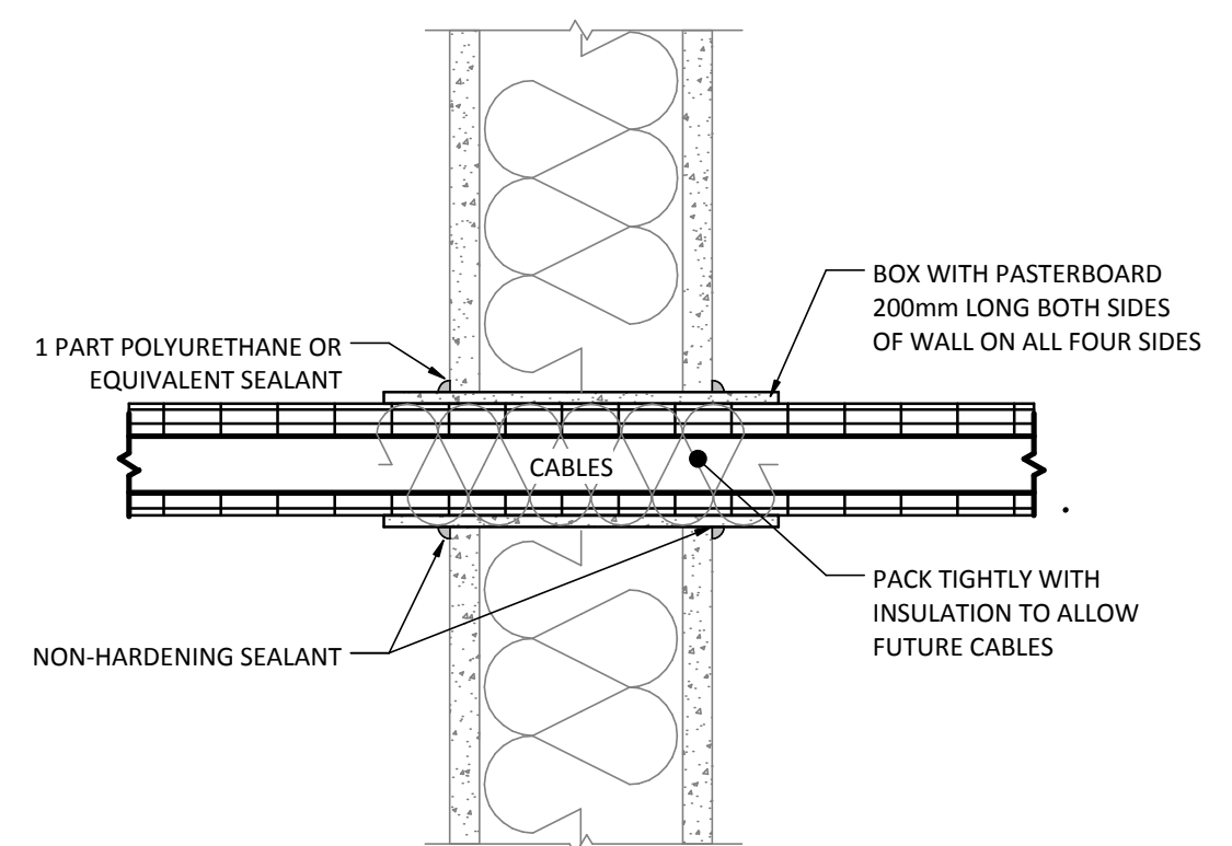
F CABLE TRAY PENETRATIONS NOT TO SCALE
