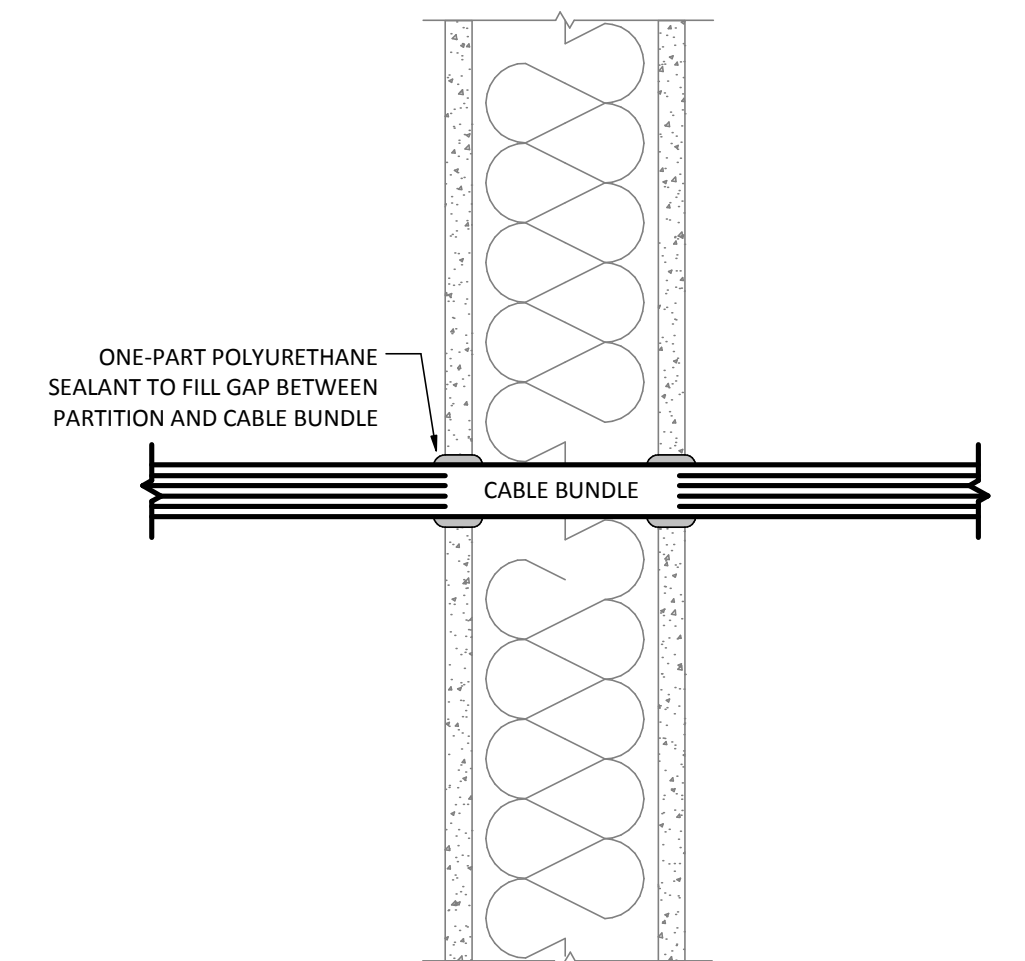
5 SEAL - HOLE IN PARTITION NOT TO SCALE
