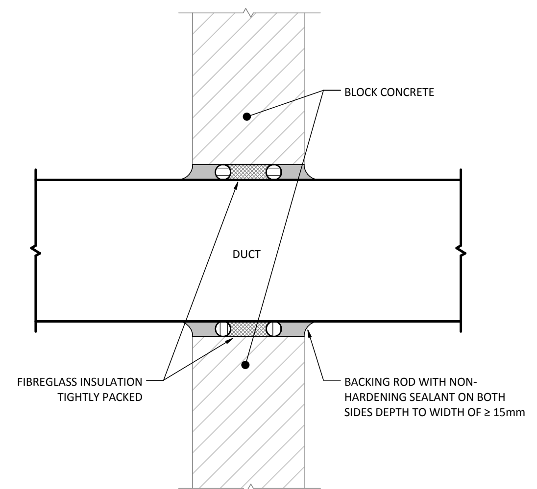
C DUCT SOLID WALL PENETRATION NOT TO SCALE
