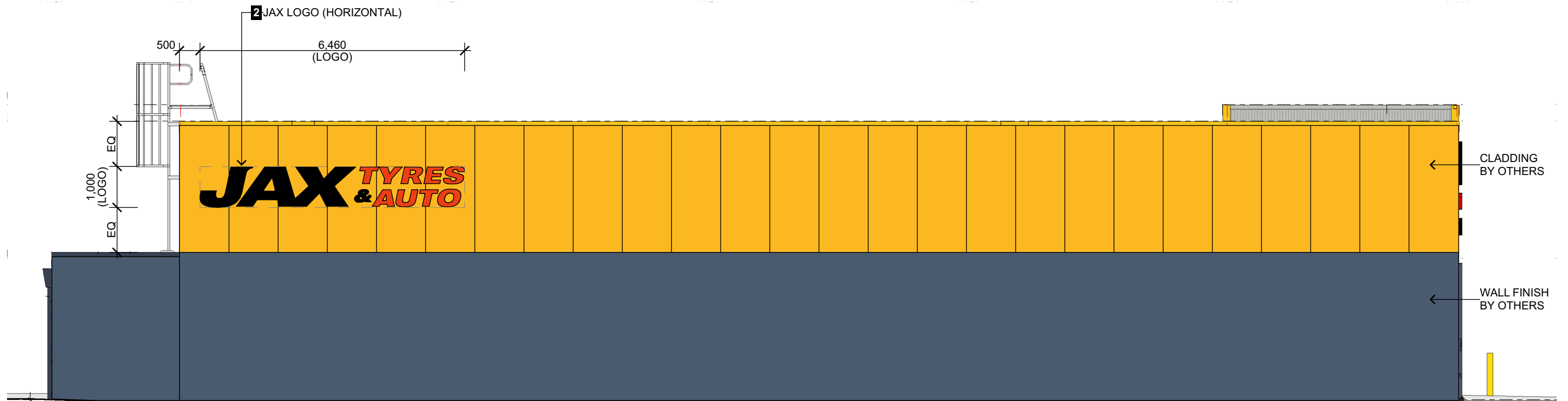
1 - ELEVATION SOUTH A3@ 1:100
