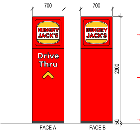
S10C 2.3m ILLUM. DIRECTIONAL SIGN 1:50
