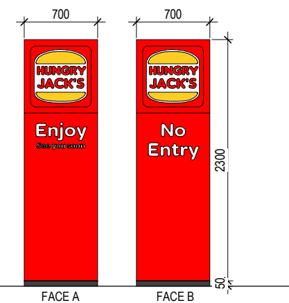
S10B 2.3m ILLUM. DIRECTIONAL SIGN 1:50
