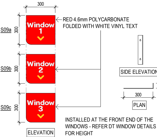
S09 DRIVE THRU BOOTH SIGN 1:20
