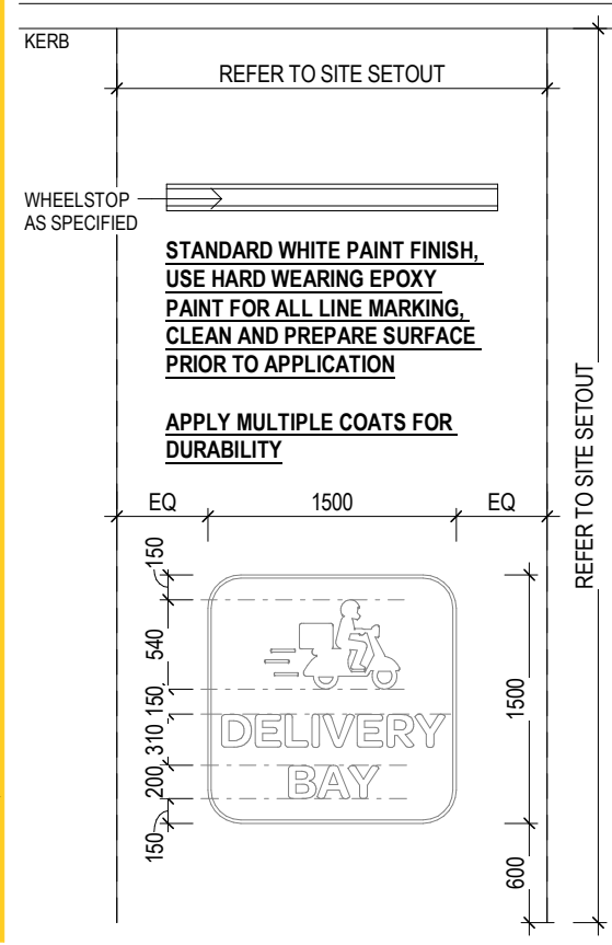
S12 DELIVERY LINEMARKING 1:50
