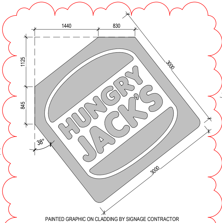
S08A ANGLED BUN GRAPHIC 1:50
