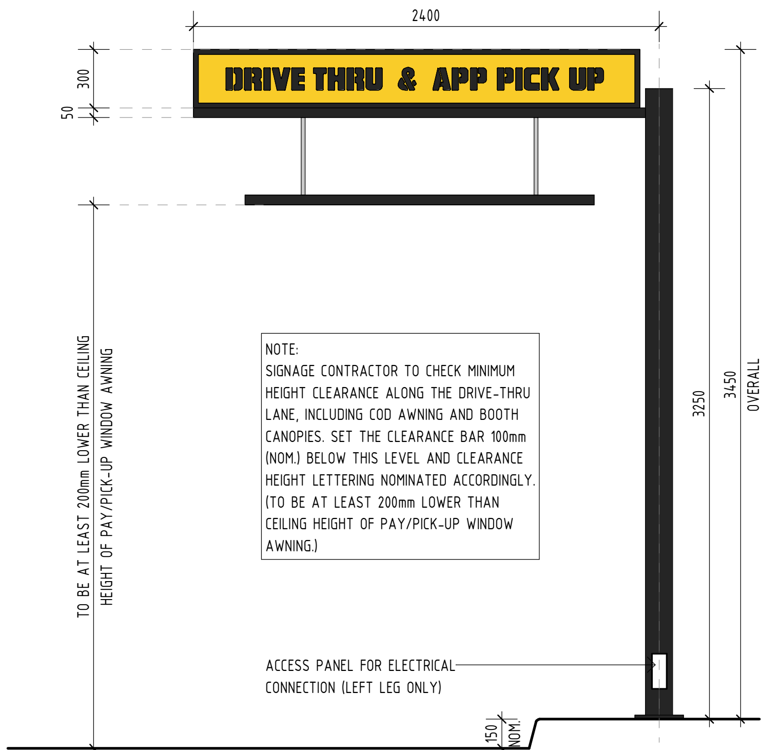
1 HB-03 - ILLUMINATED STATIC HEIGHT BAR - 2 OFF 1 : 20
