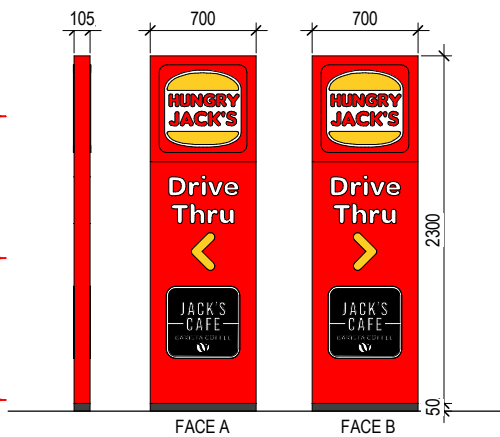
S10A 2.3m ILLUM. DIRECTIONAL SIGN 1:50
