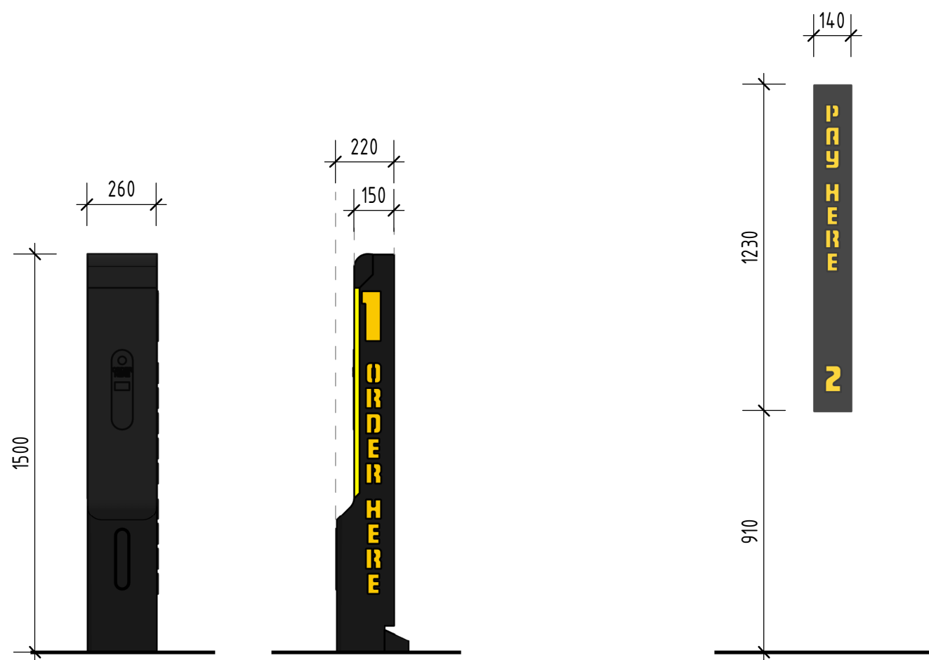
1 S14 - 1 ORDER POINT SIGN 1 : 20
