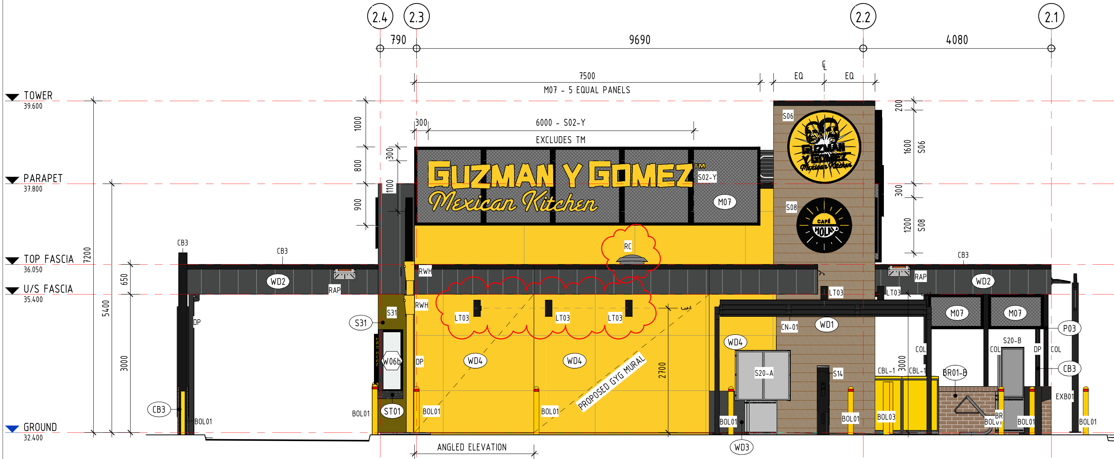
2 BUILDING ELEVATION - SOUTH-EAST 1 : 50
