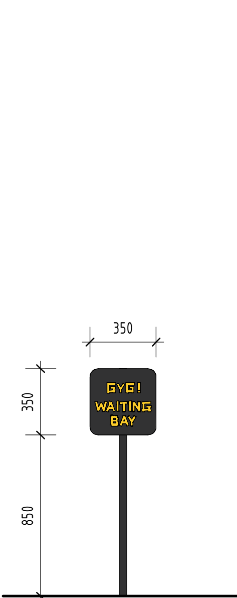
12 S35 - NON-ILLUMINATED SIGNAGE - 2 OFF 1 : 20
