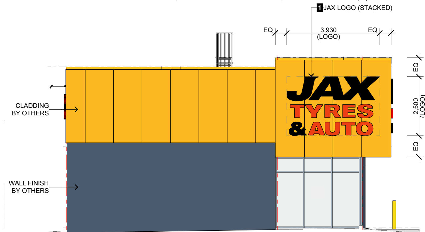
2 - ELEVATION EAST A3@ 1:100
