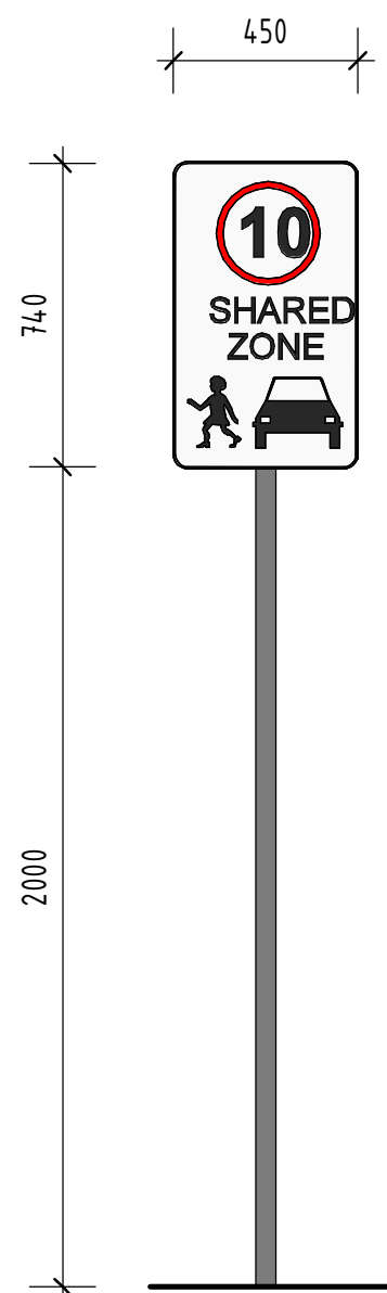
9 ST-01 - NON-ILLUMINATED SIGNAGE - 2 OFF 1 : 20
