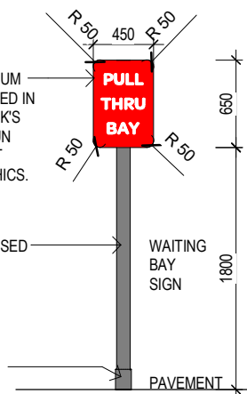
S11 WAITING BAY SIGN AND LINEMARKING 1:50
