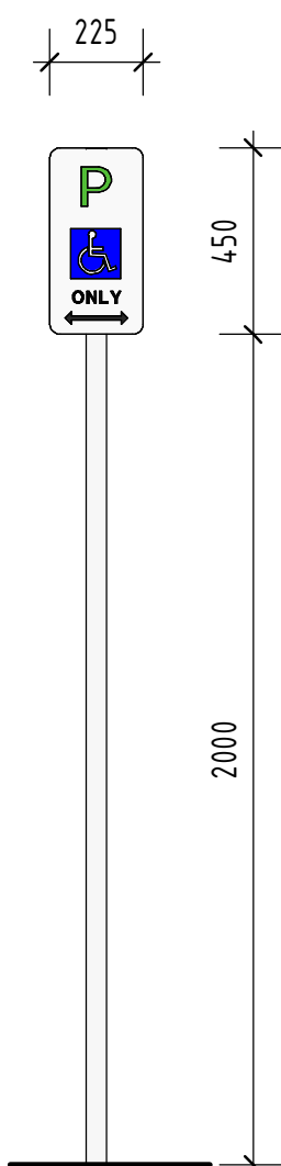
11 ST-04 - NON-ILLUMINATED SIGNAGE - 1 OFF 1 : 20
