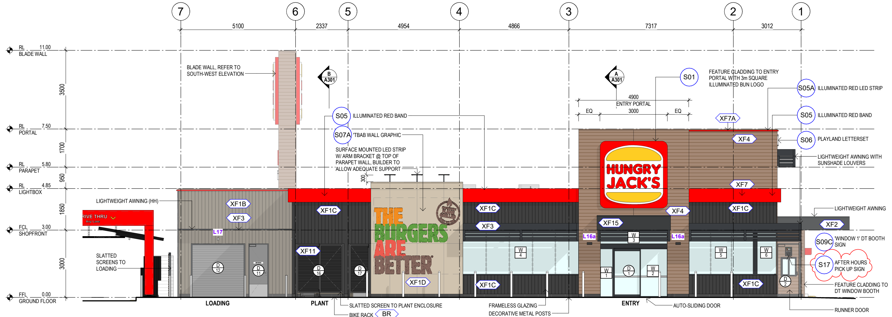
1 NORTH-EAST ELEVATION 1 : 100
