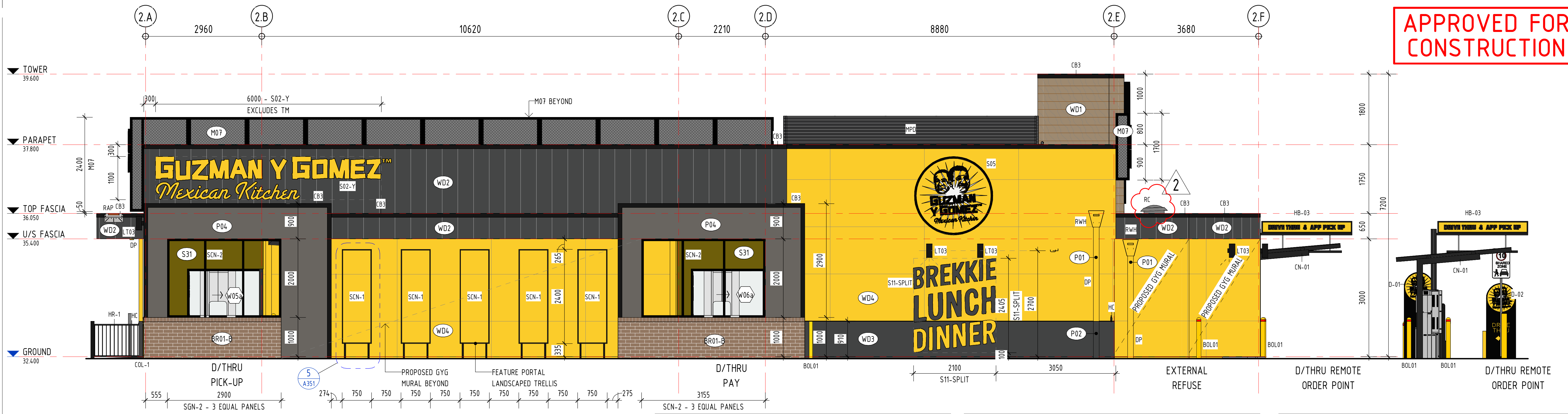
1 BUILDING ELEVATION - SOUTH-WEST 1 : 50
