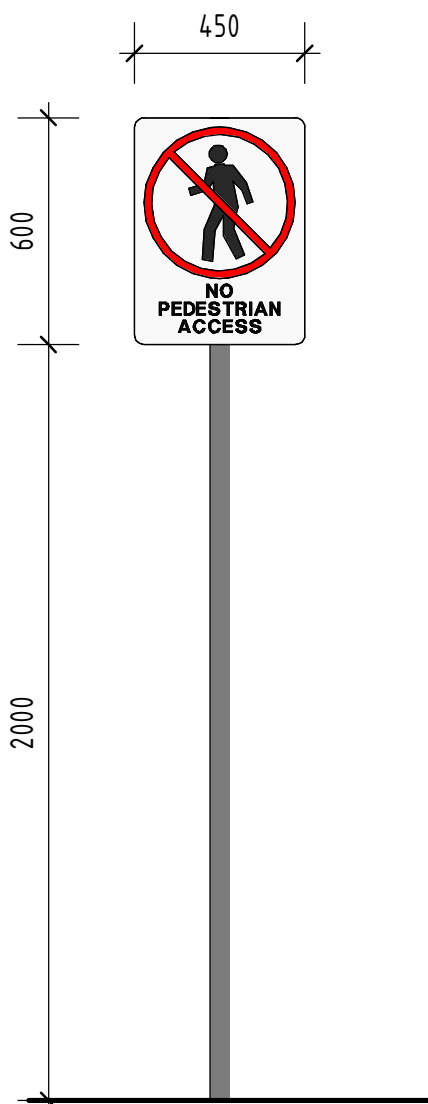
10 ST-03 - NON-ILLUMINATED SIGNAGE - 1 OFF 1 : 20
