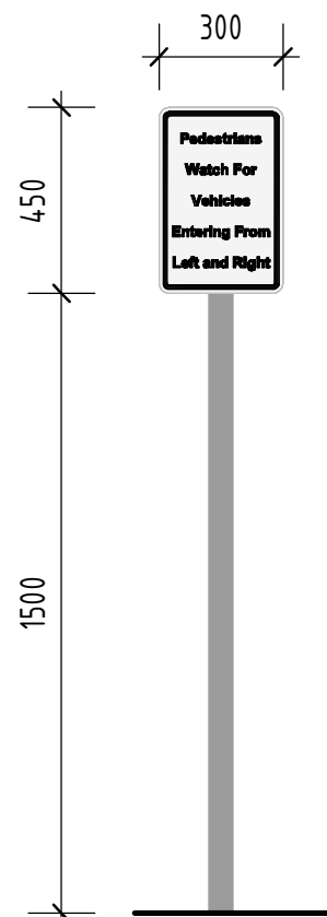
8 ST-05 - NON-ILLUMINATED SIGNAGE - 1 OFF 1 : 20
