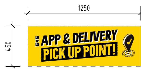
9 S19-C - NON-ILLUMINATED SIGNAGE - 1 OFF 1 : 20
