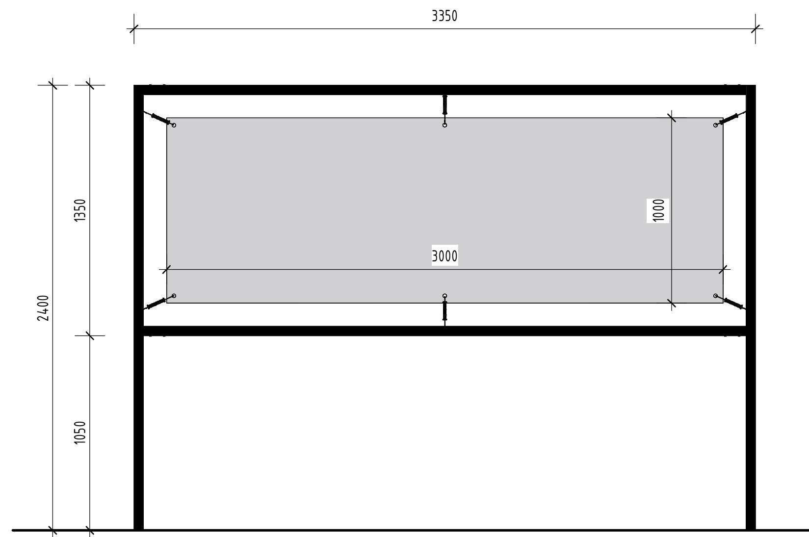
7 S36 - BREAKFAST BANNER - 1 OFF 1 : 20
