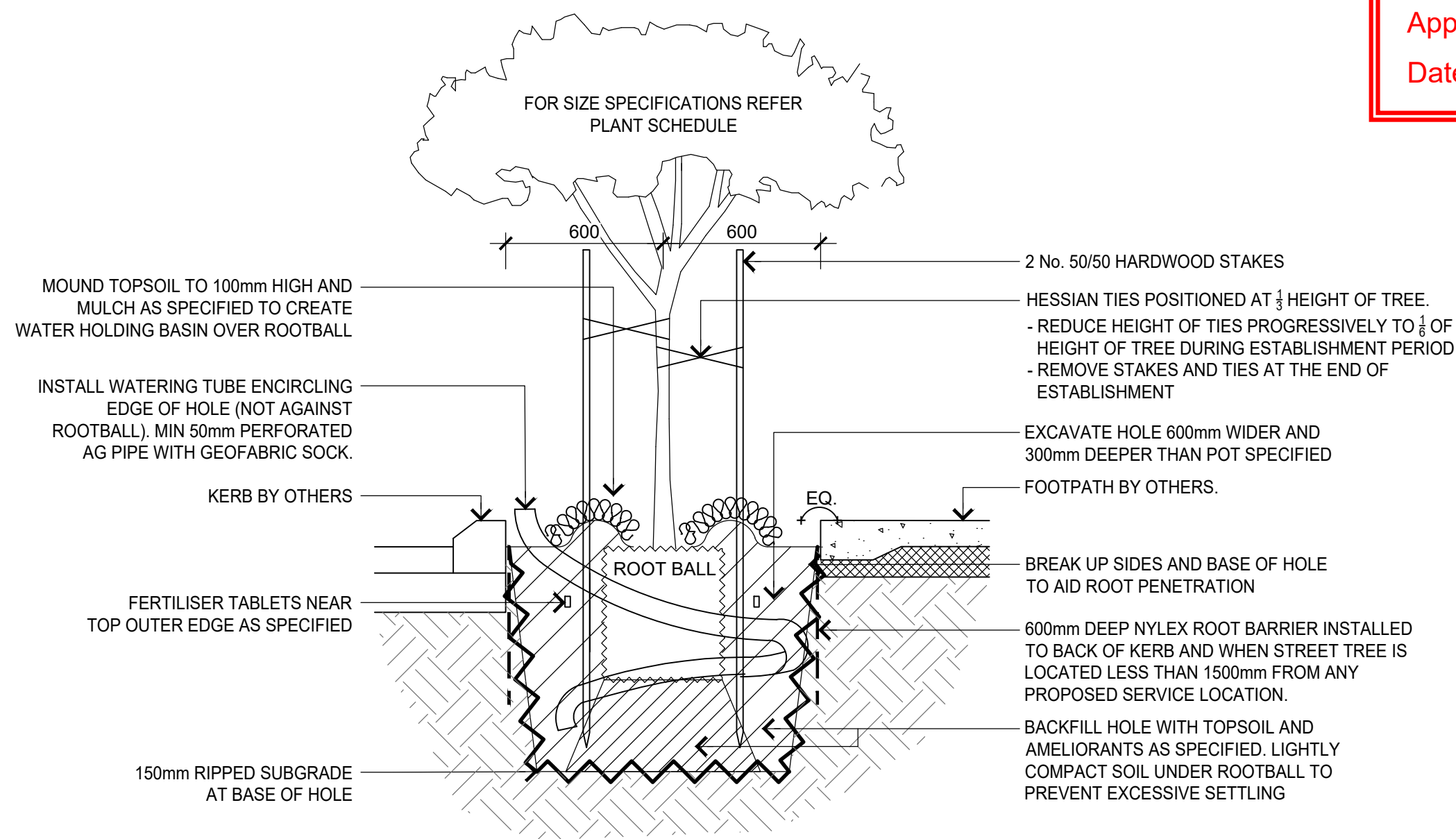
04 TREE TO THE BACK OF KERB WITH ROOT BARRIER 800 1:20 @ A1
