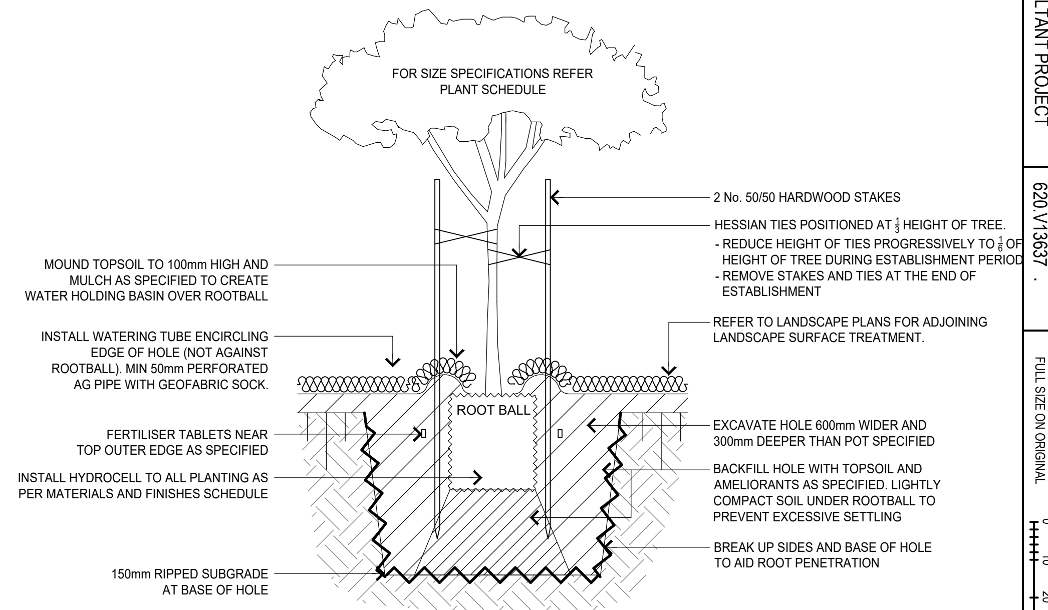
02 TREE IN GARDEN BED 800 1:20 @ A1
