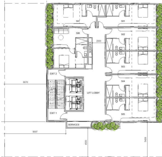
5 TH - 15 TH TYPICAL FLOOR PLAN
