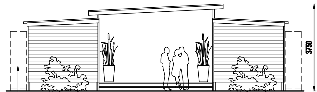
PROPOSED END ELEVATION BLOCK OF 8 UNITS
