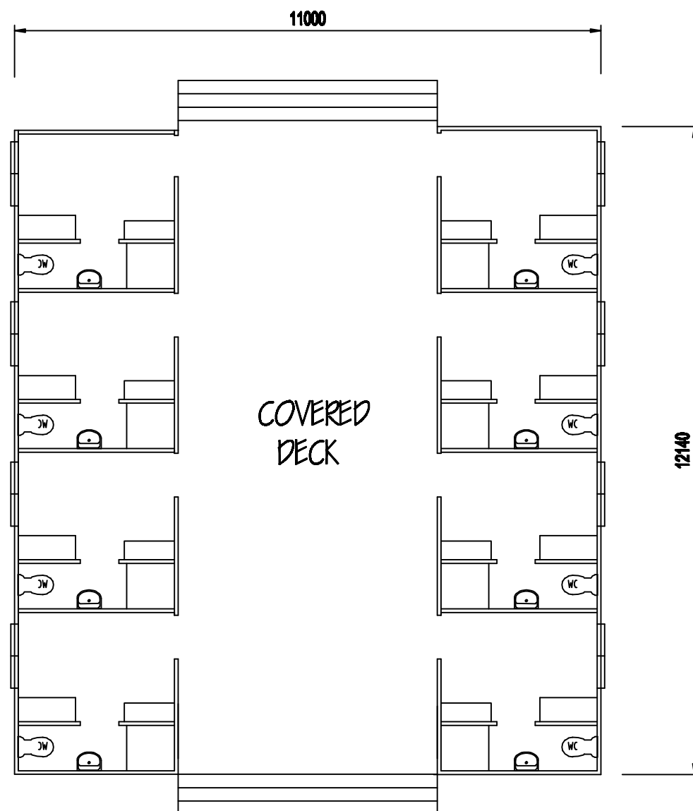
PROPOSED TYP BLOCK OF 8 UNITS
