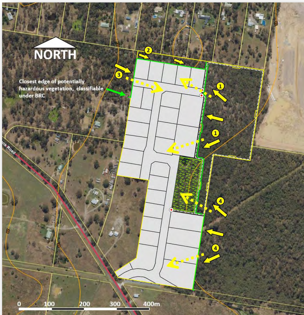
Figure 4. Vegetation and slope combinations for three main fire scenarios
