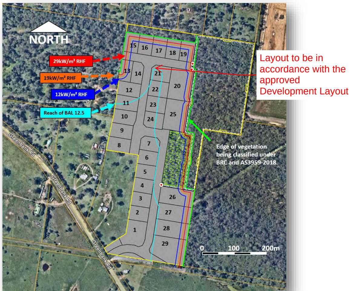
Figure 13. RHF Contours for the site
