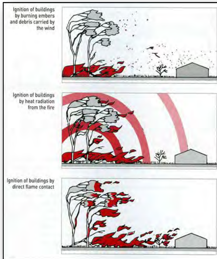
Figure 10. Main Bushfire Attack mechanisms (Image courtesy of Ramsay & Rudolf, 2003)
