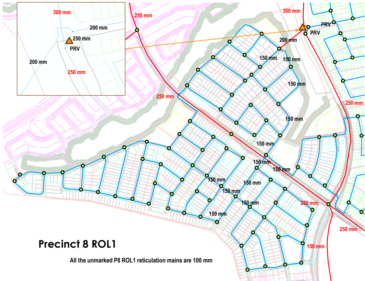
Figure 3: Proposed Precinct 8 ROL1 Water Reticulation Mains
