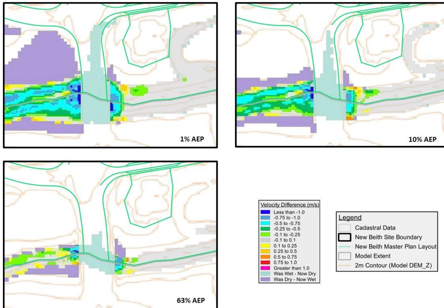
Figure 25 Flagstone Creek Crossing – Velocity Changes
