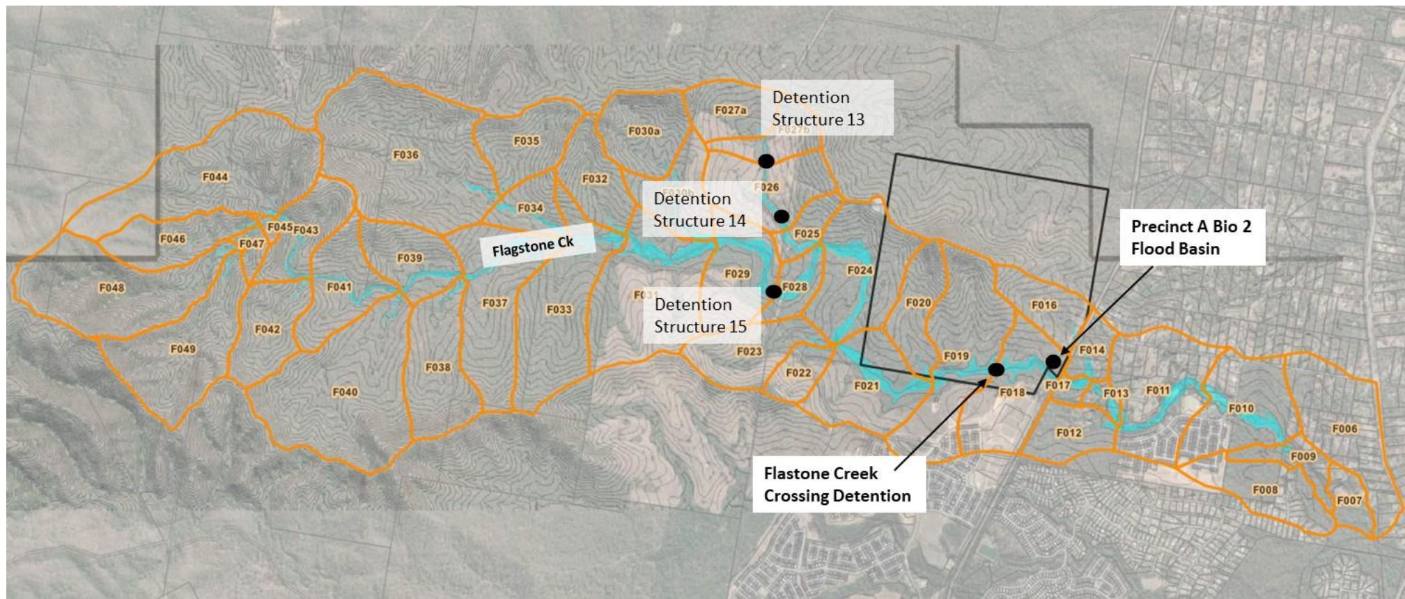
Figure 10 Location of flood detention systems – Ultimate Development
