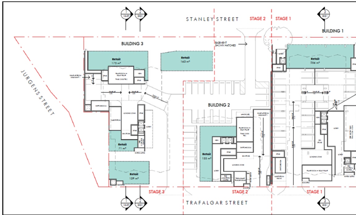
FIGURE 2 – GROUND FLOOR
