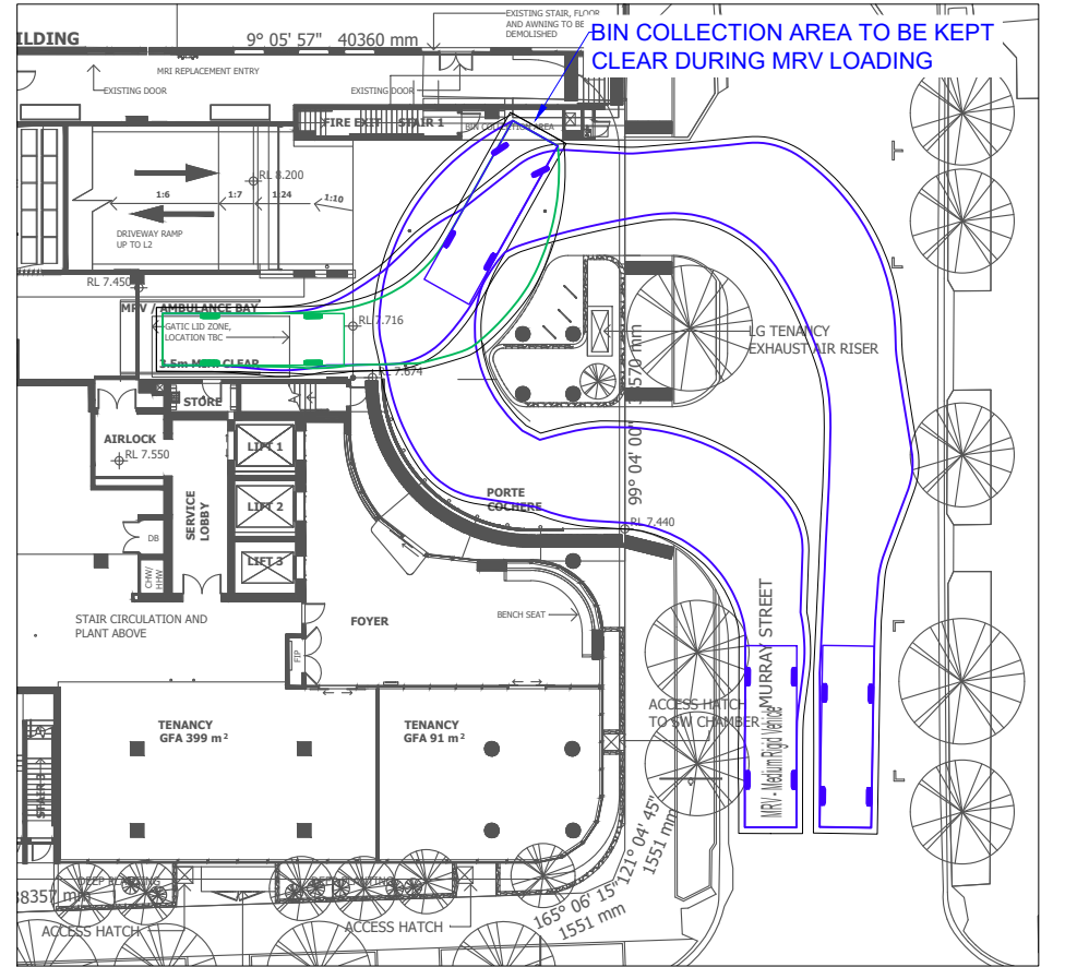
8.8m MEDIUM RIGID VEHICLE (MRV) INGRESS/EGRESS MANOEUVRE
