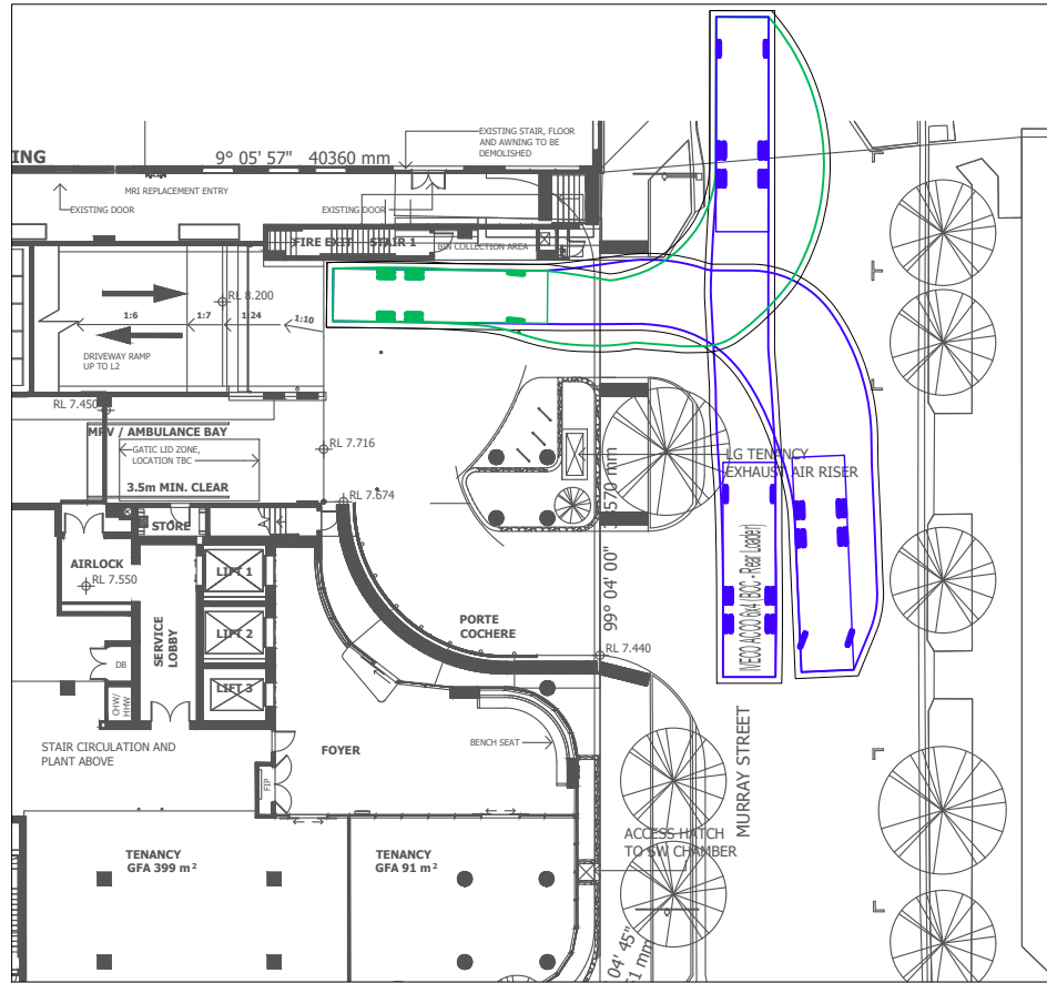
10.23m REFUSE COLLECTION VEHICLE (RCV) INGRESS/EGRESS MANOEUVRE
