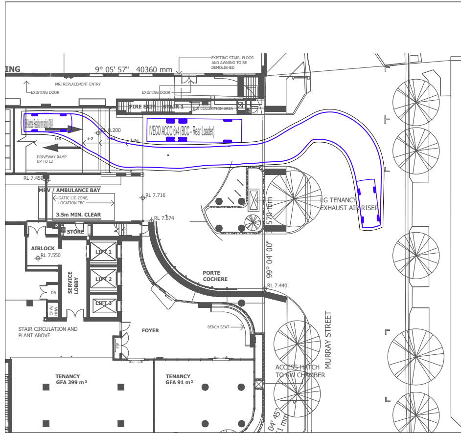
B99 EGRESS PASSING A 10.23m REFUSE COLLECTION VEHICLE (RCV)
