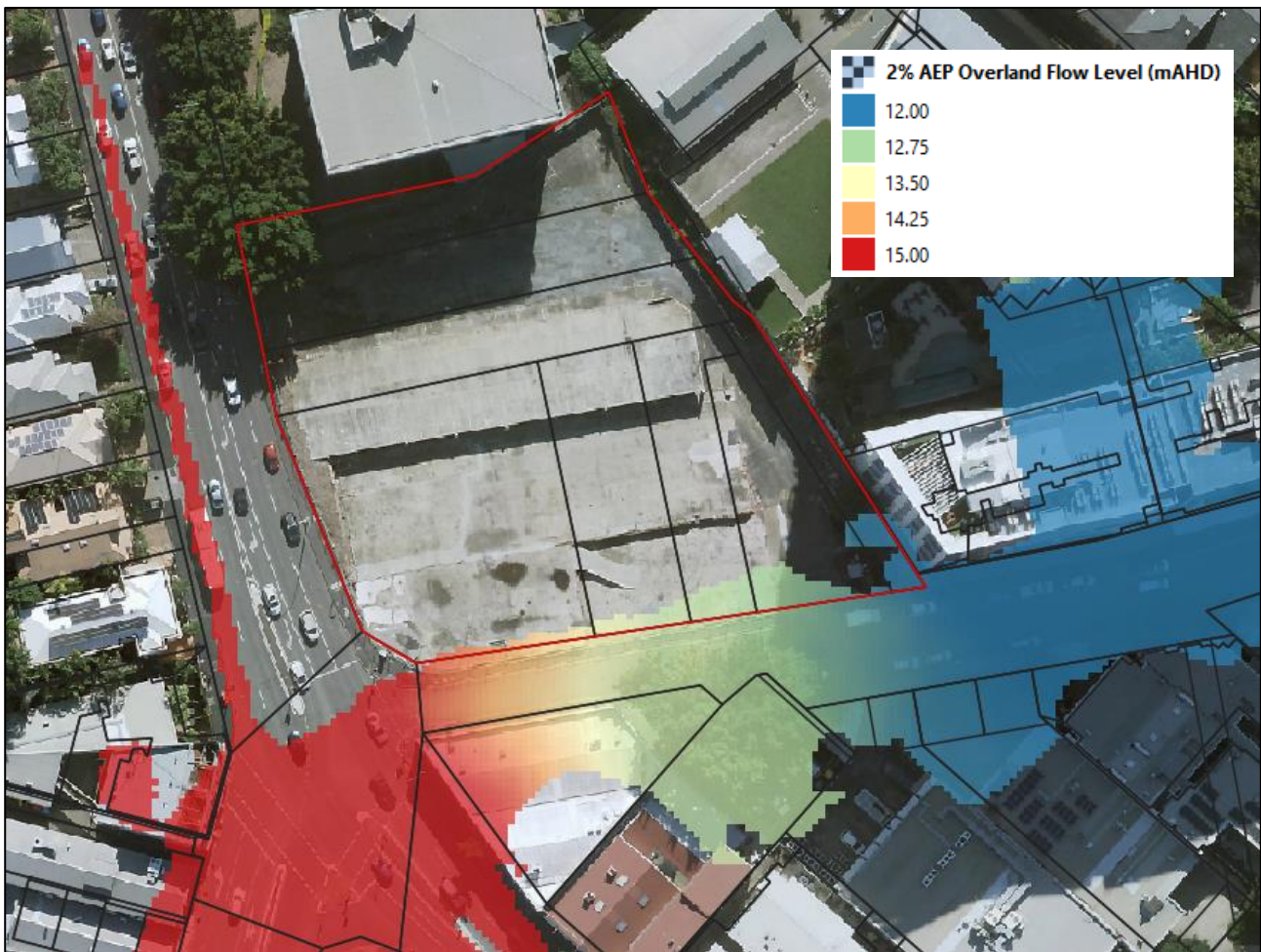
Figure 3.2 2% AEP Peak Overland Flow Flood Level (BCC, 2019)
