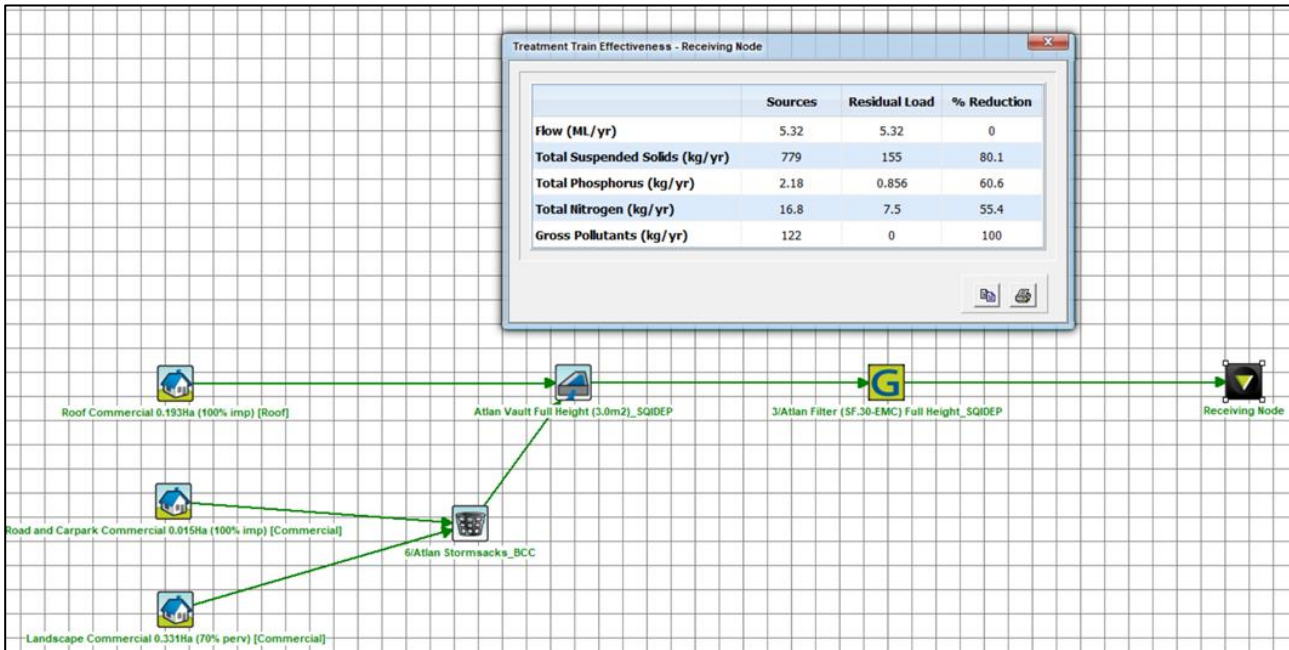
Figure 4.2 Treatment Train Layout & MUSIC Results
