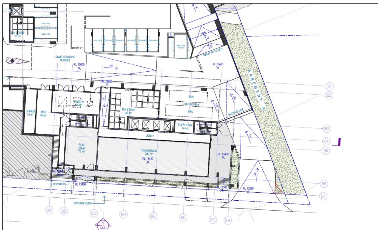
Figure 3.3 Proposed Basement Carpark Entrance Level (Woods Bagot, 2023)
