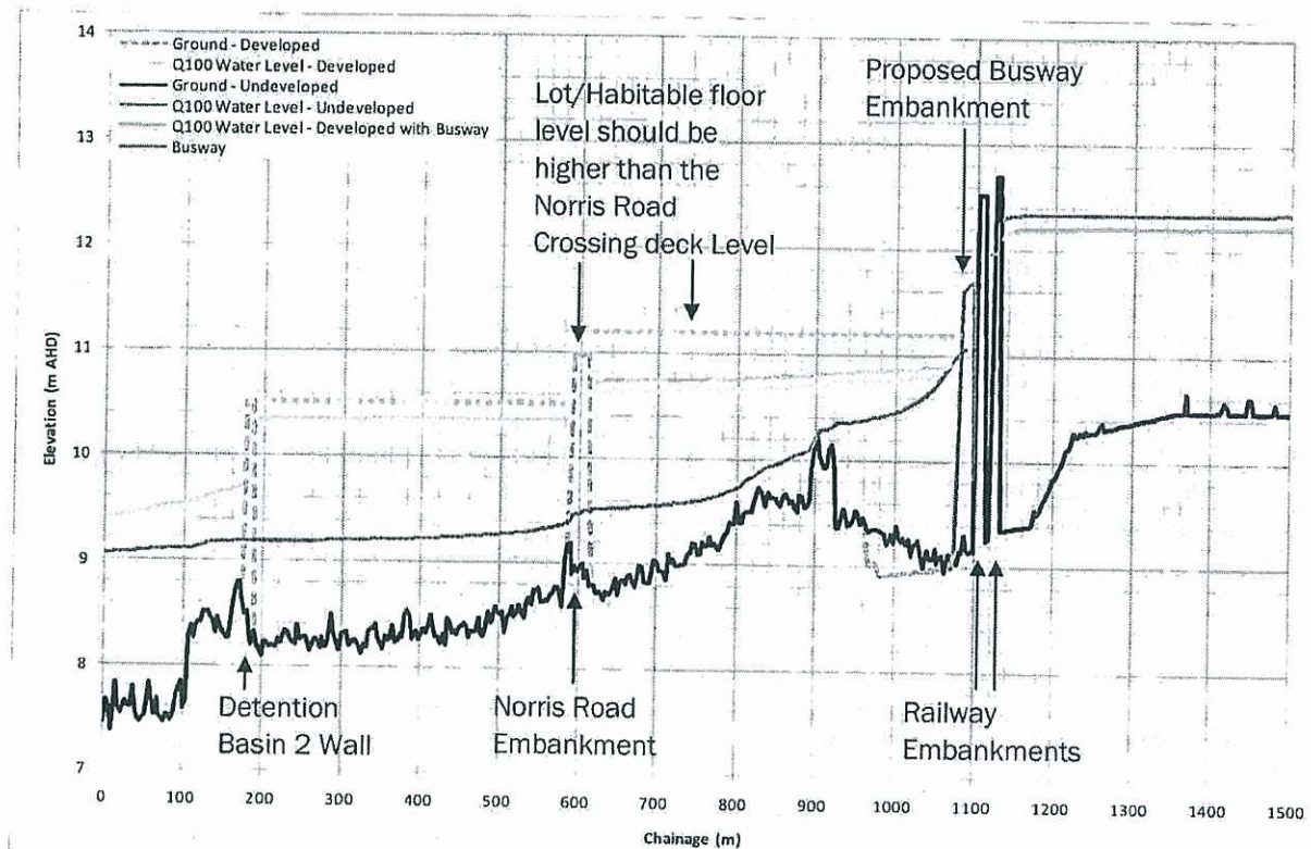
Figure 6 Long Section of Undeveloped and Developed Carseldine Drain 100 Year ARI Water Levels
