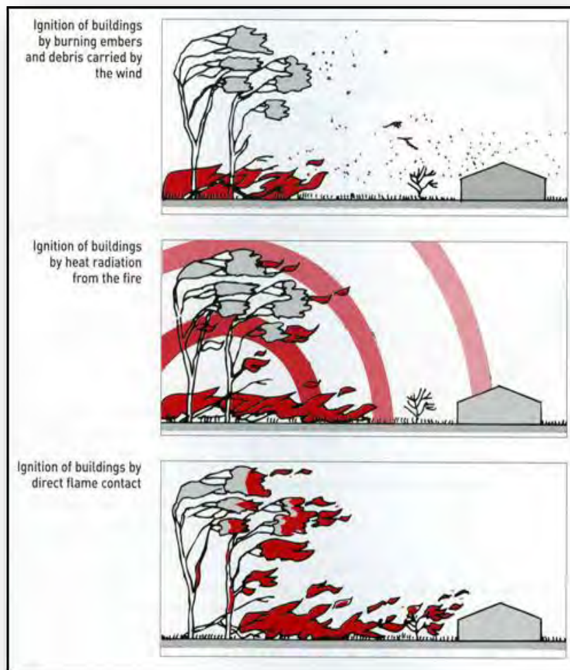
Figure 8. Main Bushfire Attack mechanisms (Image courtesy of Ramsay & Rudolf, 2003)
