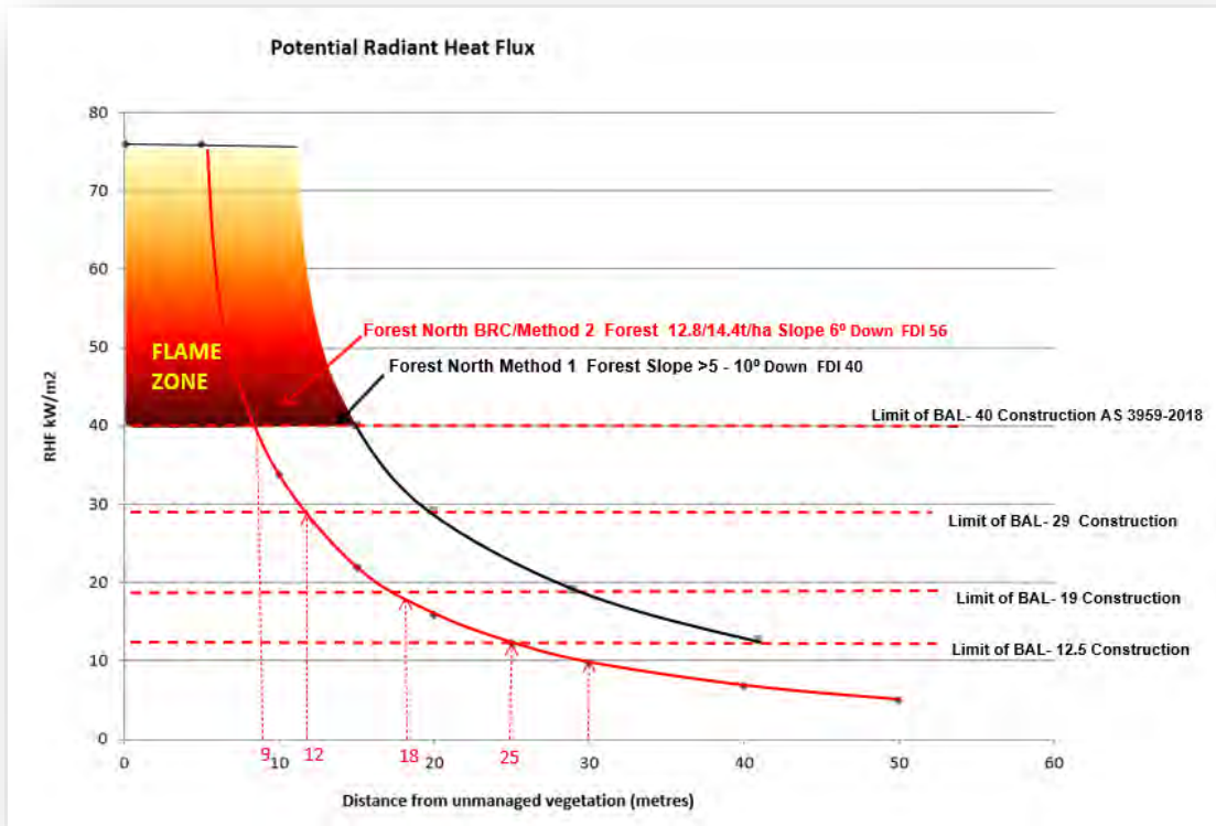
Figure 9. Radiant Heat Flux Predicted by Methods 1 and 2.
