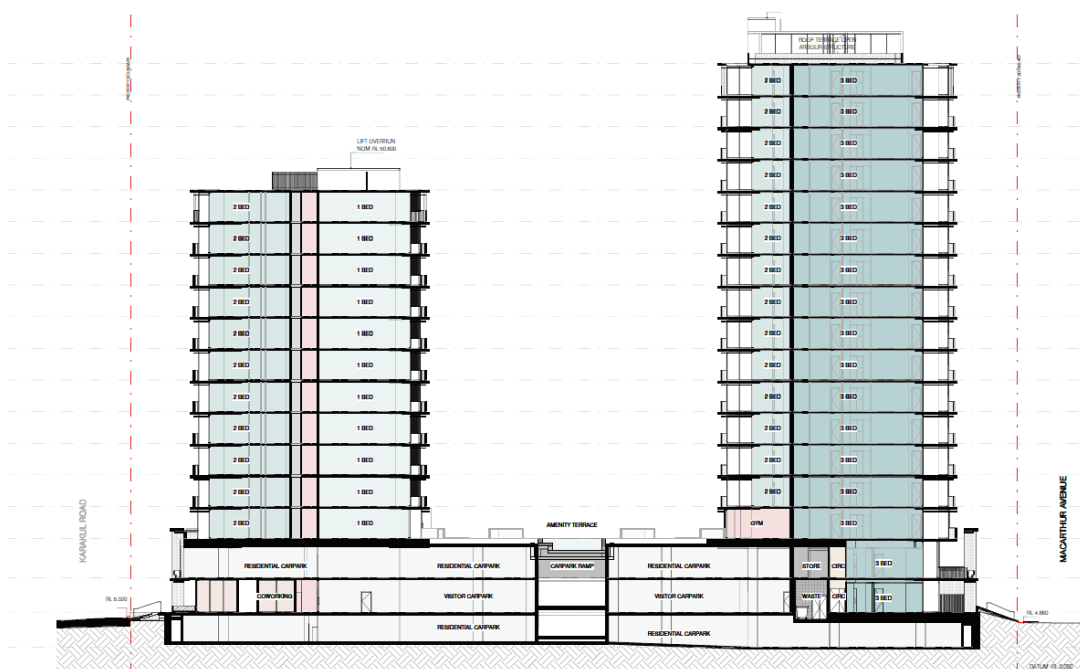
Image 5: Extract from proposed development Section plan (Carr 24047-TP3-3001).
