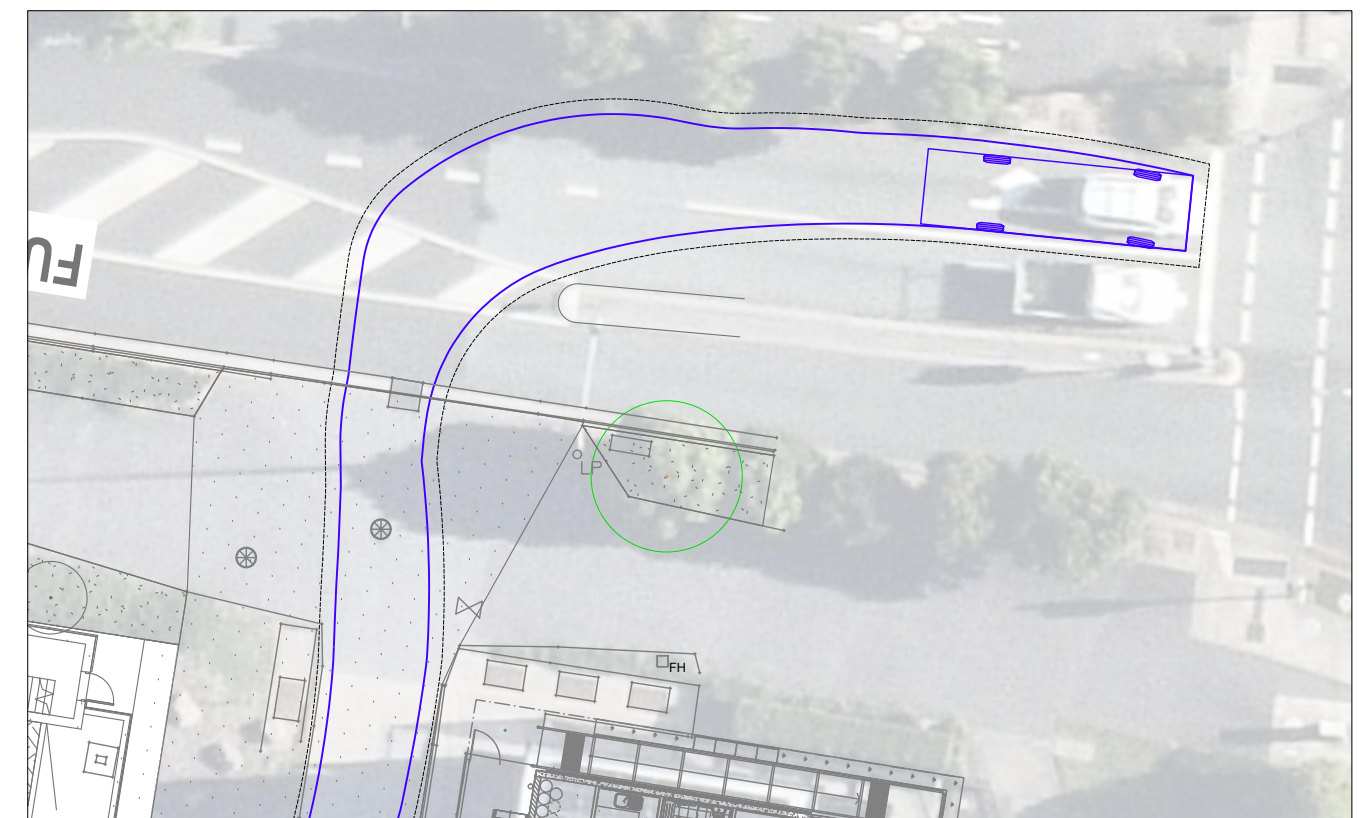
NORTH ACCESS DRIVEWAY LAYOUT SCALE 1:250
