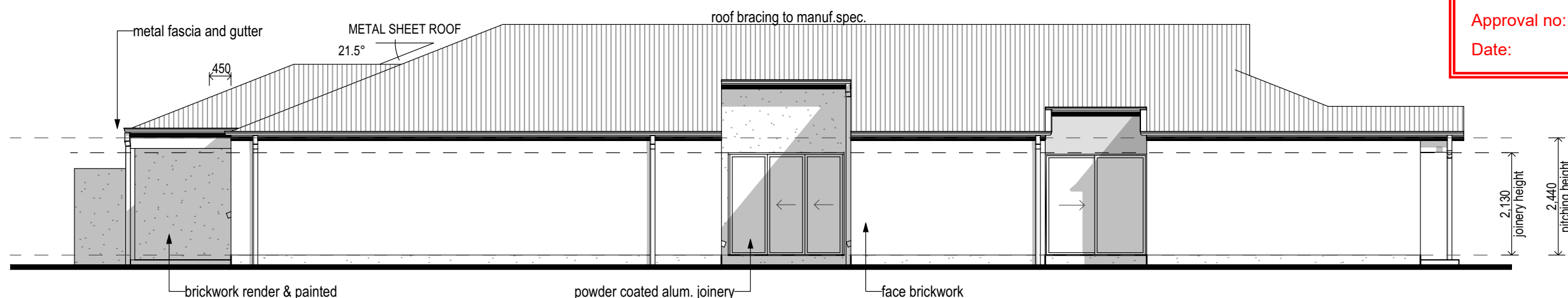
Elevation 4 Scale 1:100
