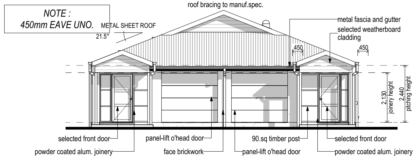
Elevation 1 Scale 1:100
