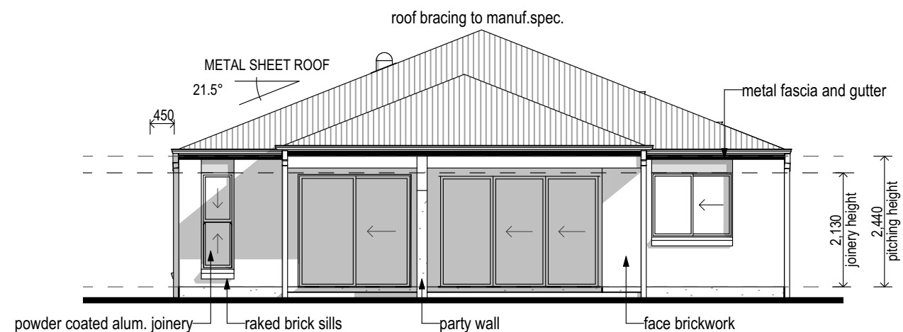
Elevation 3 Scale 1:100
