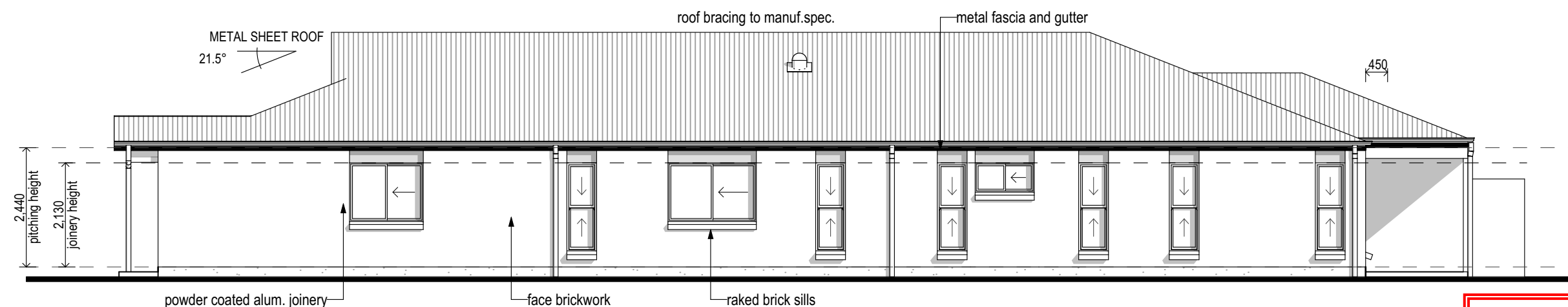
Elevation 2 Scale 1:100
