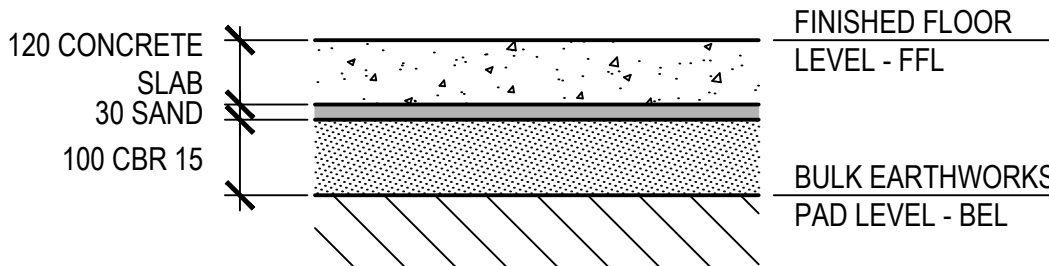
BUILDING WORKING PLATFORM DETAIL N.T.S.
