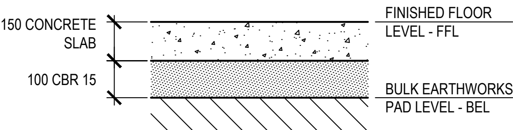
CAR PARK WORKING PLATFORM DETAIL N.T.S.
