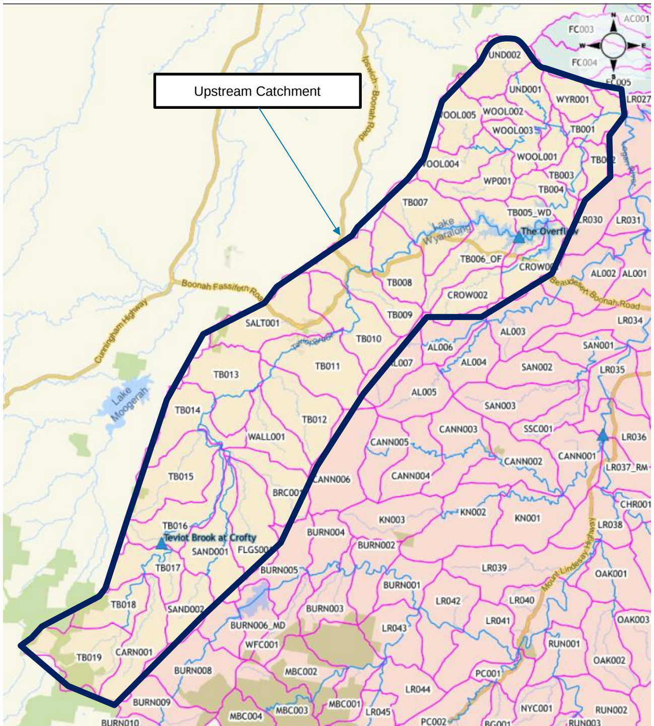
Figure 5-3 Upstream Sub-Catchments from LARFS (2023)
