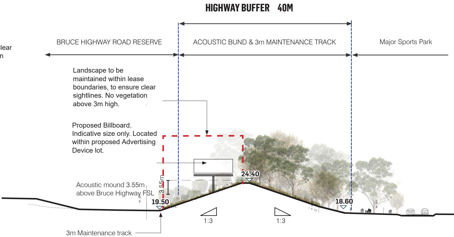
SECTION 01 1:250 @ A1 1:500 @ A3 2.5 5 7.5 10 12.5m
