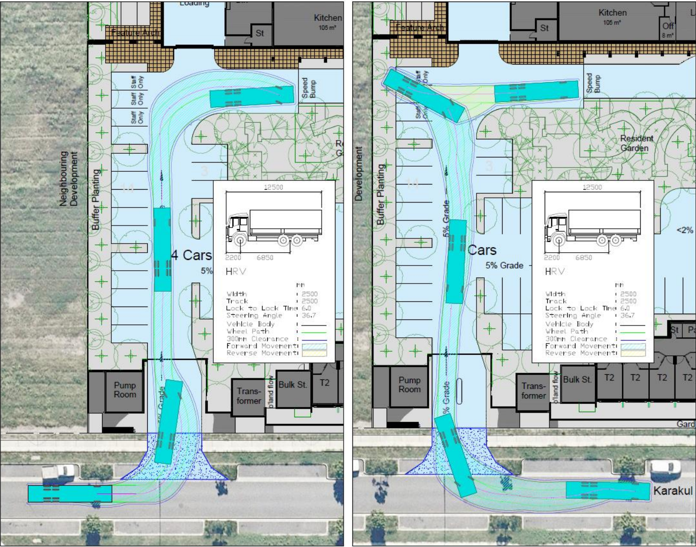
FIGURE 6.3 – SWEEP PATHS FOR A HEAVY RIGID VEHICLE (HRV)
